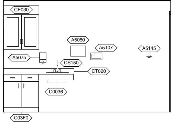
XDUS1 - EAST ELEVATION
