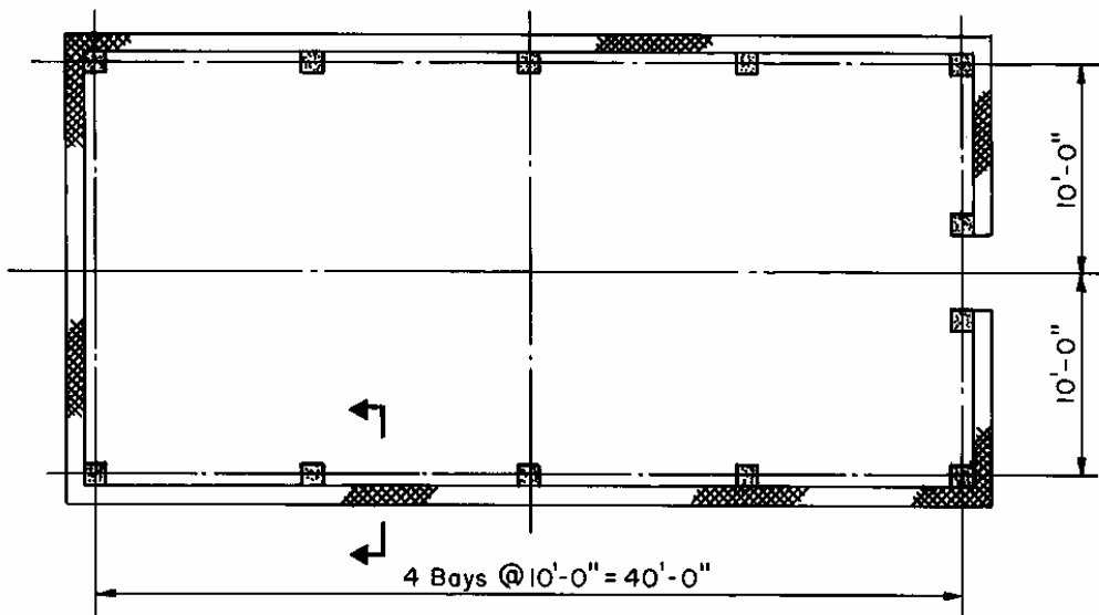
FLOOR PLAN
