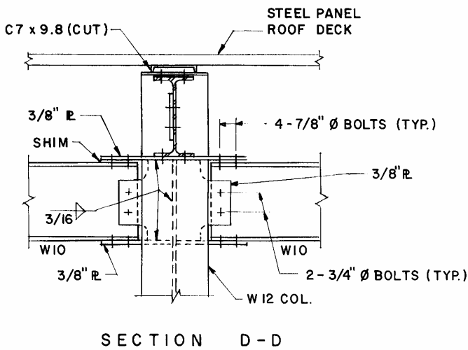
Figure 5-33 Typical framing detail at end Column 1-C
