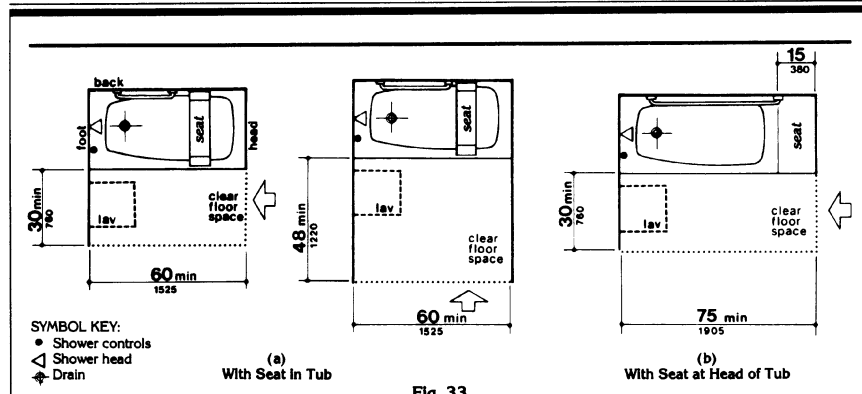
Fig. 33 Clear Floor Space at Bathtubs
