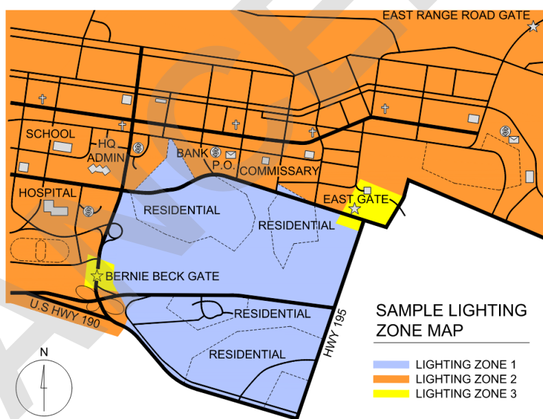
Figure 4-1 Example Lighting Zones on a Sample Installation
