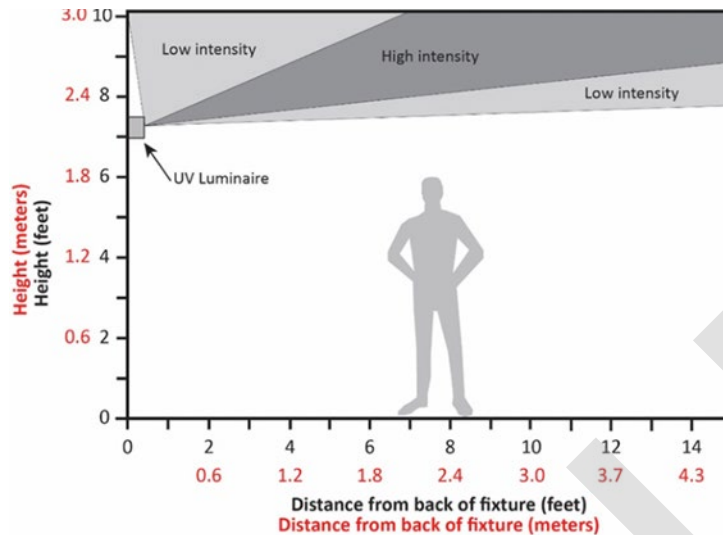
Figure E-2 Upper-Air UV Installation (www.ies.org)
