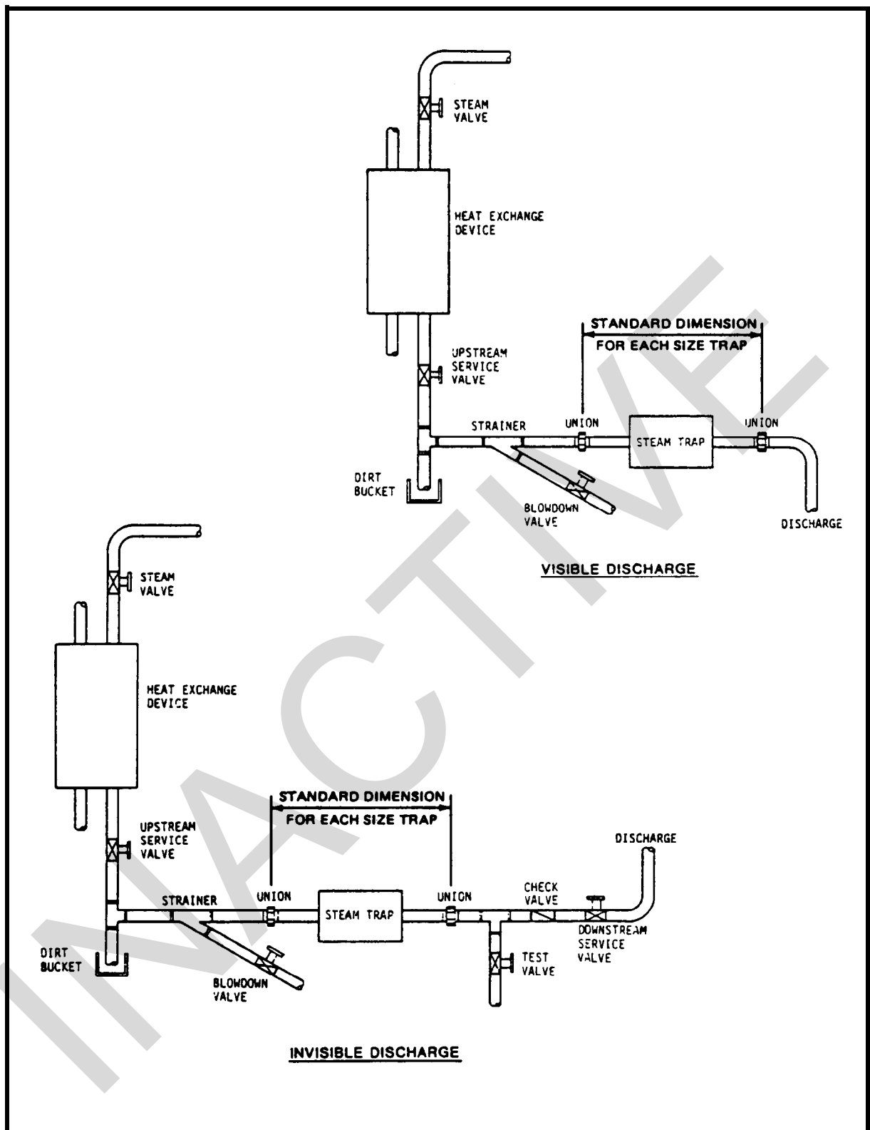
FIGURE 3-9. Typical Steam Trap Installations
