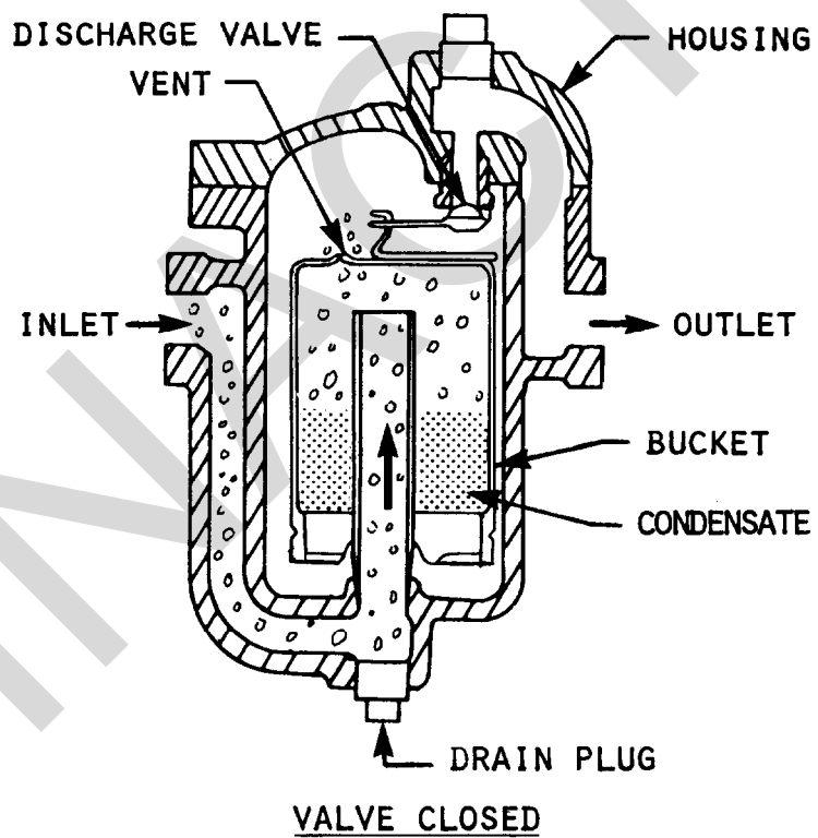
FIGURE 8-2. Inverted Bucket Trap
