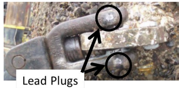
Figure 2-32 Lead Plugs Securing the Riser Swivel Shackle
