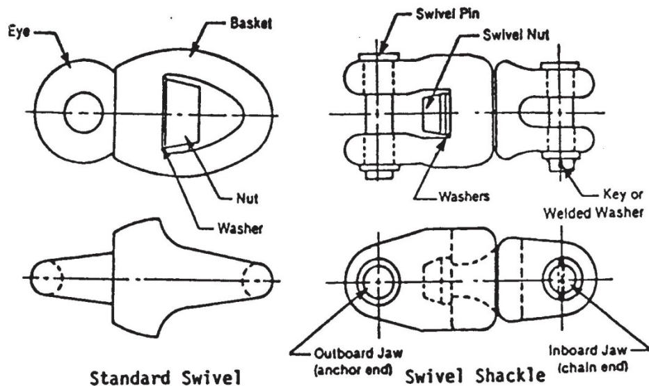
Figure 2-30 Swivel Fittings
