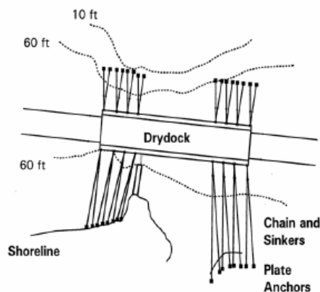
Figure 2-5 Spread Mooring
