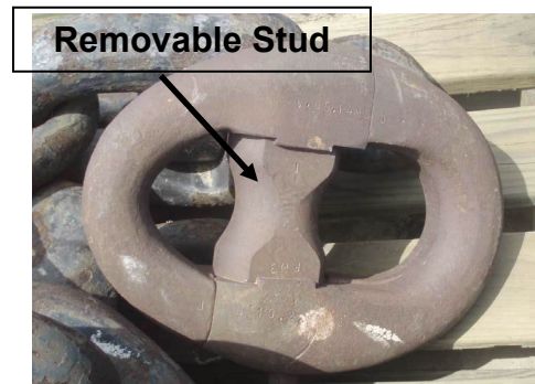
Figure 2-26 Kenter Style Anchor Joining Link
