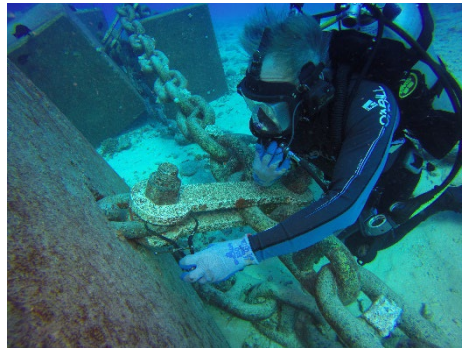
Figure 2-39 Plate Shackle Attaching Sinkers to Chain
