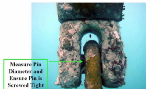
Figure 3-36 Bottom of Riser Swivel Shackle by Chain
