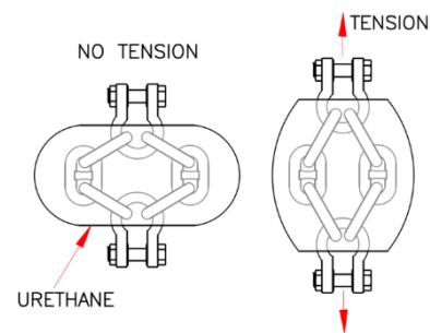
Figure 2-45 Kinetic Link Details
