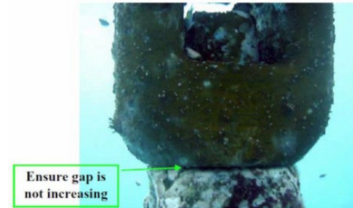
Figure 3-35 Cleaning and Inspection of Swivel Gap
