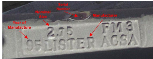
Figure 3-25 Pear Link Marking Data
