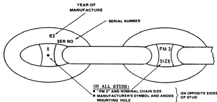
Figure 6-5 Chain Markings
