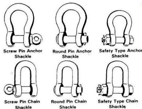
Figure 2-34 Shackles
