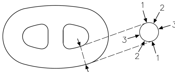
Figure 3-10 Single Link Measurement
