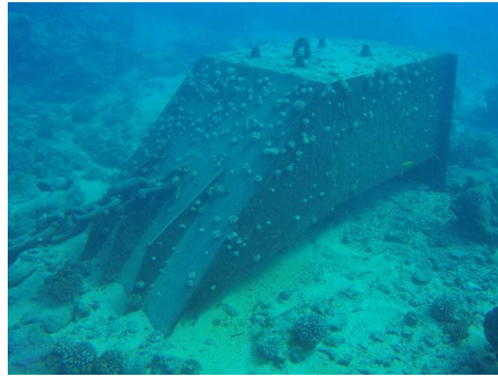
Figure 2-20 Pearl Harbor Style Deadweight Anchor
