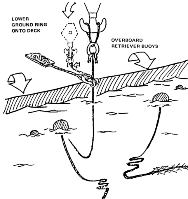
Figure K-3 Two Anchor Chain Subassemblies Overboarded
