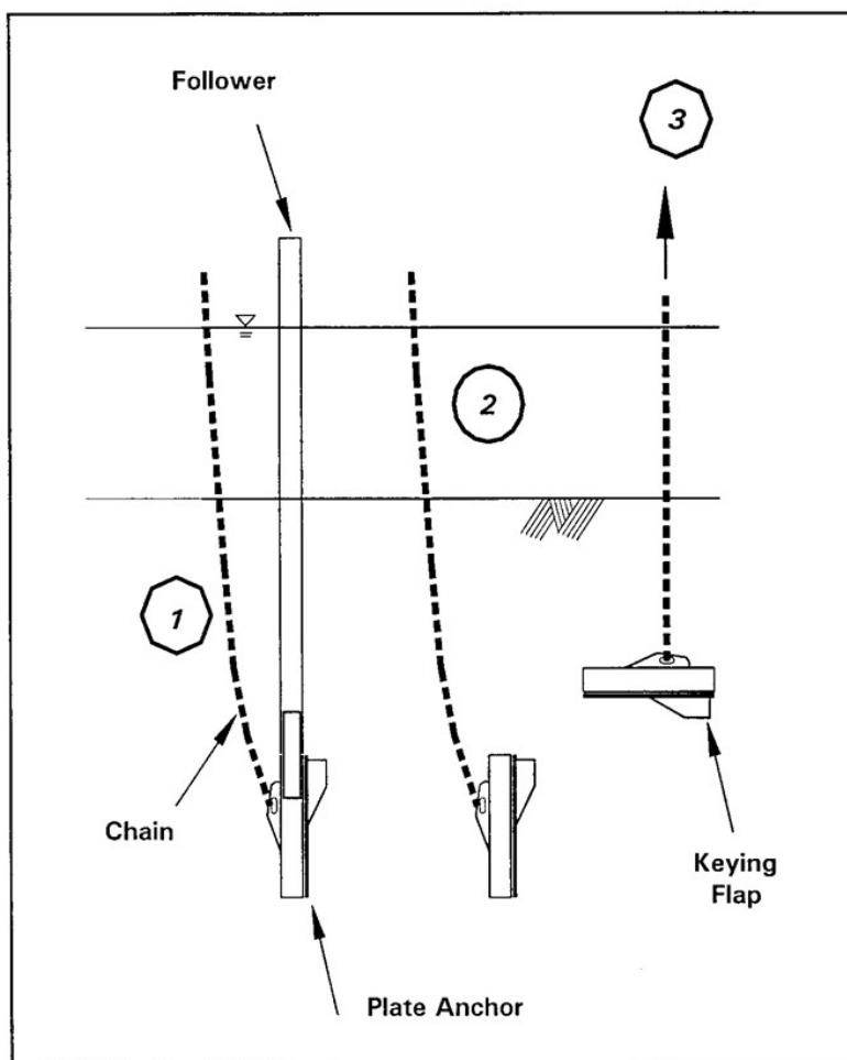
Figure 2-16 Plate Anchor
