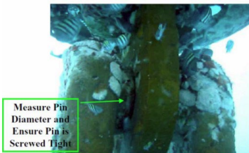
Figure 3-34 Top of Riser Swivel Shackle by Buoy
