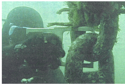
Figure 3-9 Double Link Measurement at a Chain Link Joint
