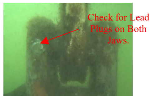
Figure 3-37 Lead Plugs in Riser Swivel Shackle Jaw
