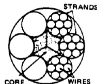
Figure 2-53 Wire Rope Structure
