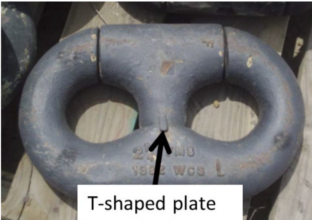
Figure 2-23 Baldt Style Chain Joining Link
