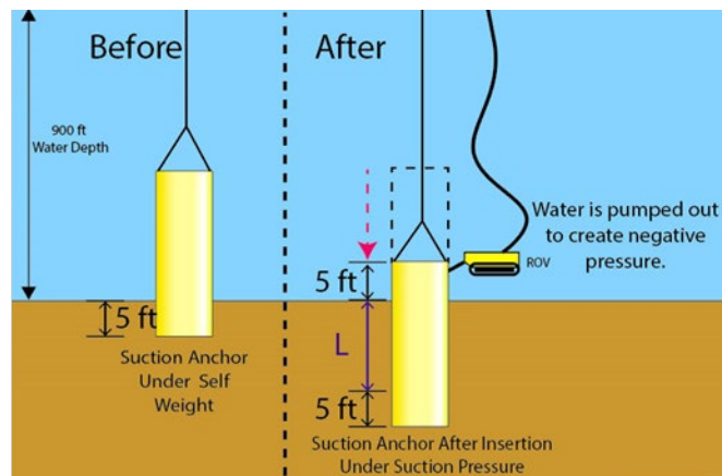
Figure 2-17 Suction Anchor
