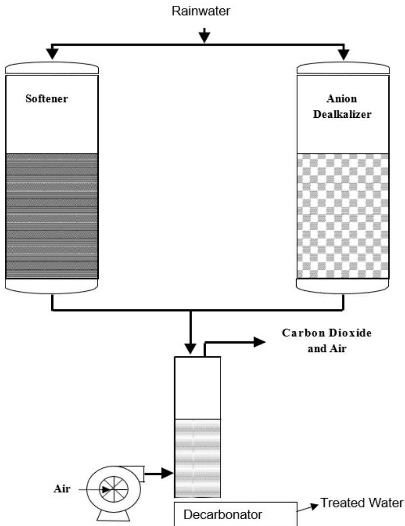
Figure 3-6 Split-Stream Dealkalizer
