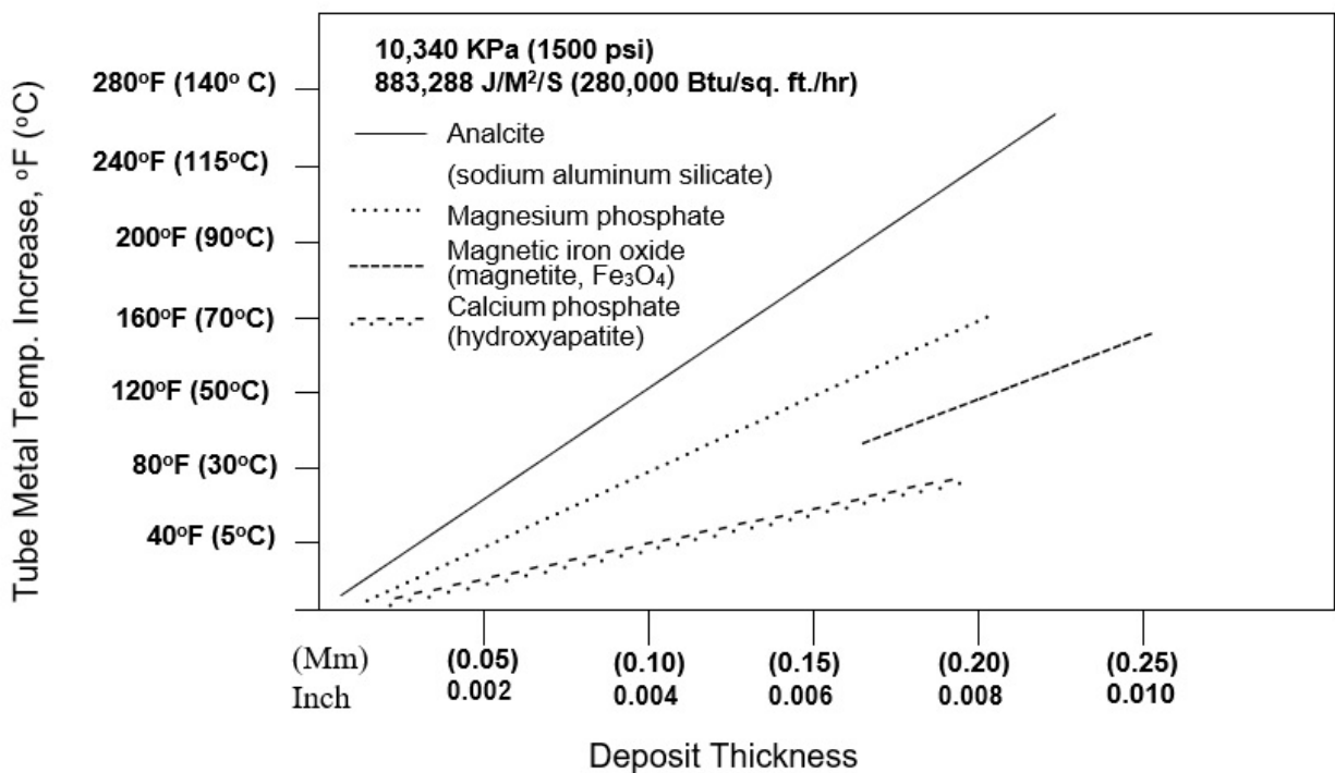
Figure 4-6 Impact of Scale on Heat Transfer
