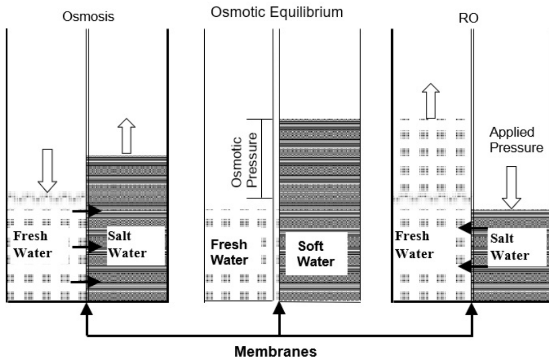
Figure 3-7 RO Schematic
