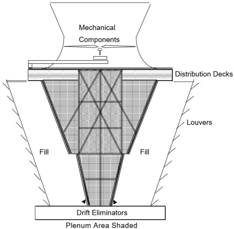
Figure 5-6 Cross-Flow Cooling Tower
