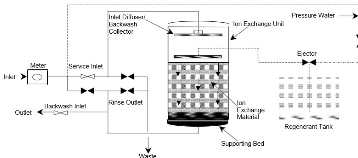
Figure 3-2 Typical Ion Exchange Unit
