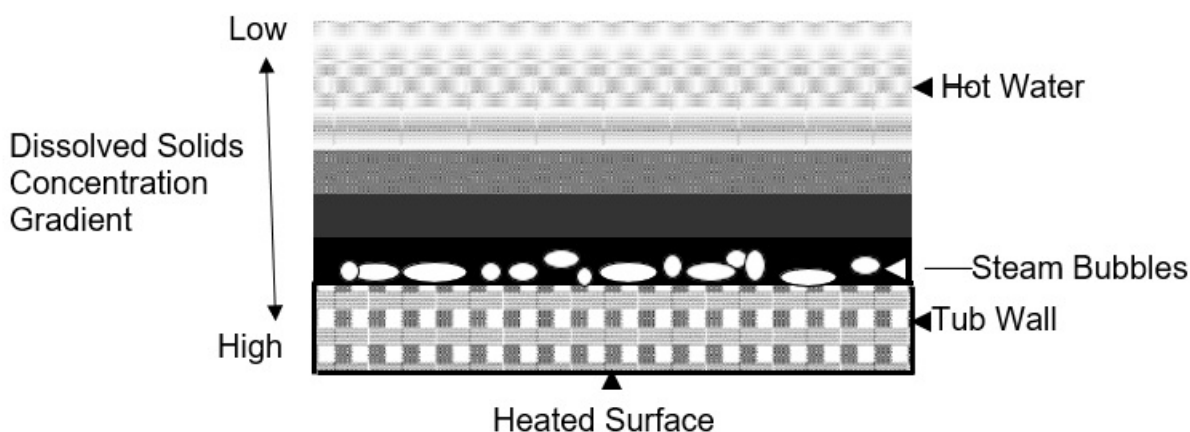
Figure 4-11 Localized Scale Formation Process
