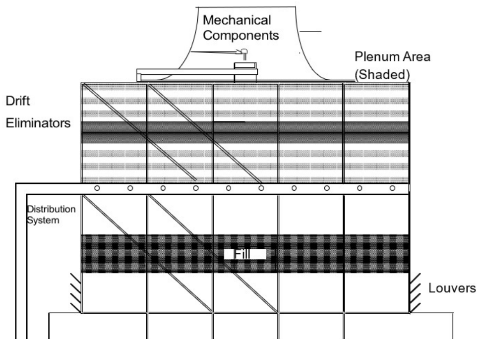
Figure 5-8 Counter-Flow Cooling Tower Diagram
