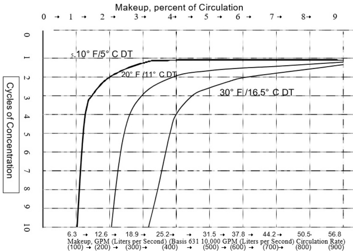
Figure 5-15 Effect of COC on Makeup Requirement
