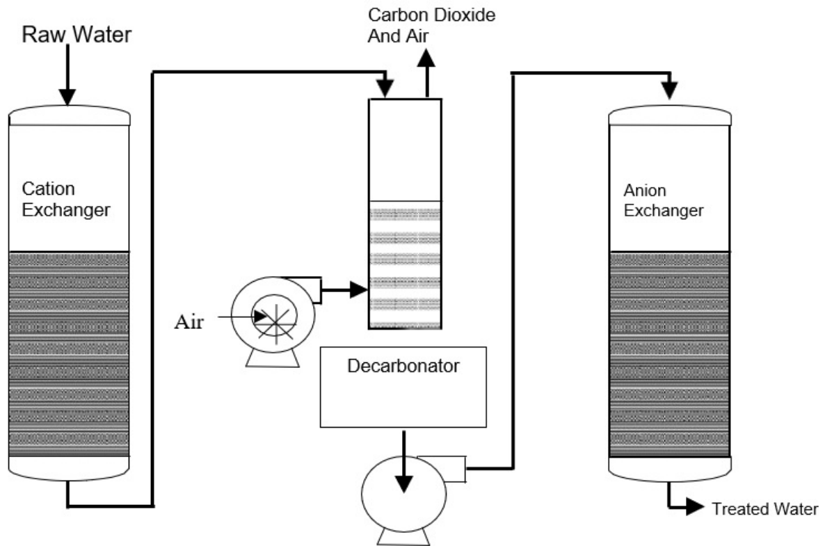
Figure 3-4 Demineralization Process
