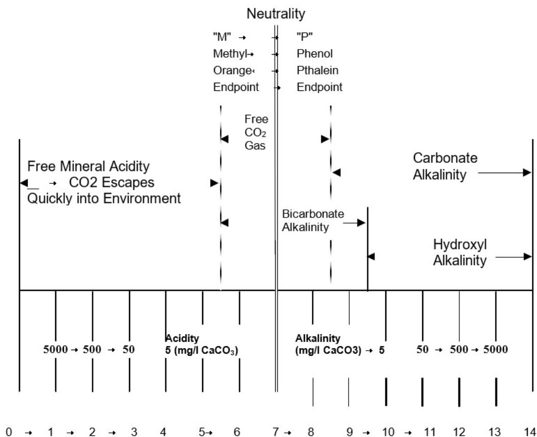
Figure 7-4 Acidity, Alkalinity, and pH Ranges.
