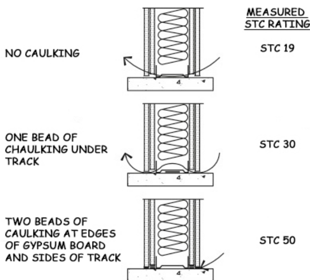
Figure 3-5 Sealing Tracks
