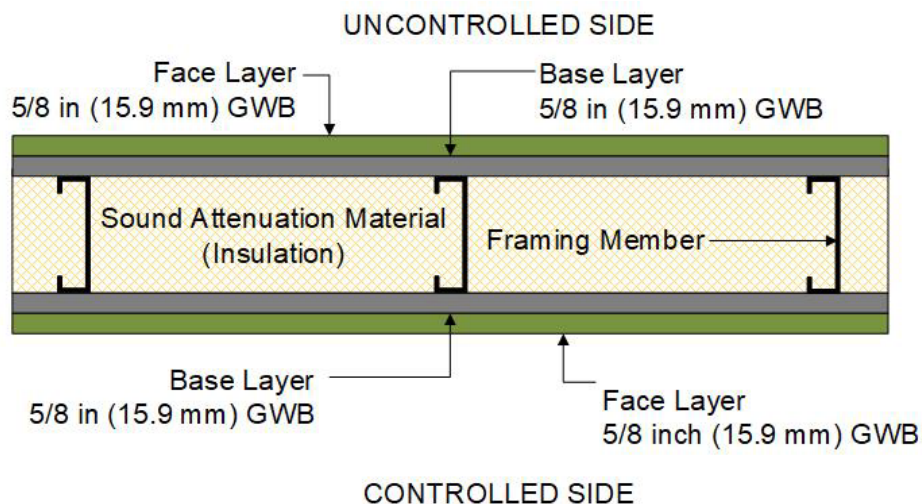
Figure 3-4 STC 50 Assembly
