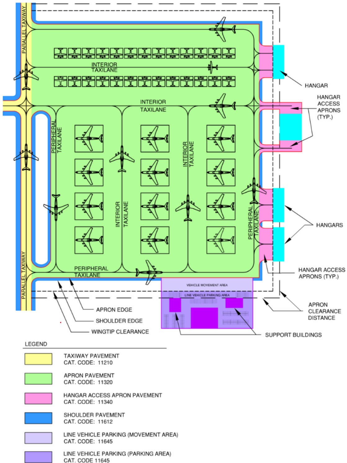
Figure 11320-2 Apron and Taxiway Category Codes
