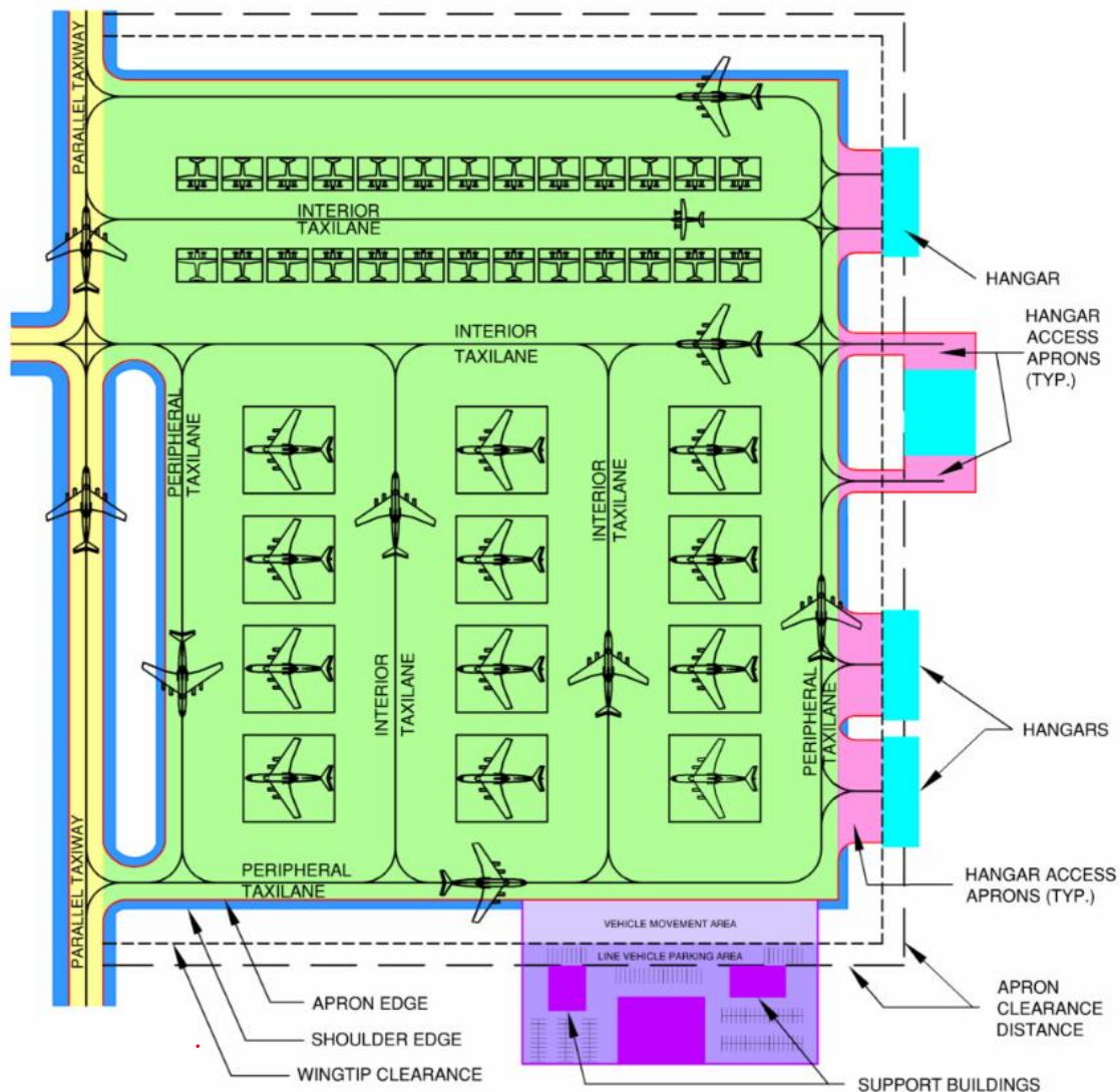
Figure 11320-2 Apron and Taxiway Category Codes
