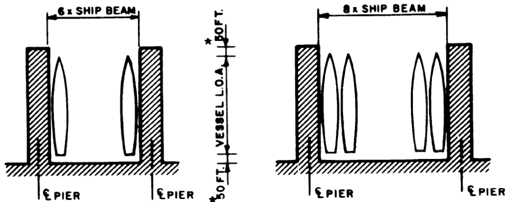
TWO-ABREAST BERTHING
