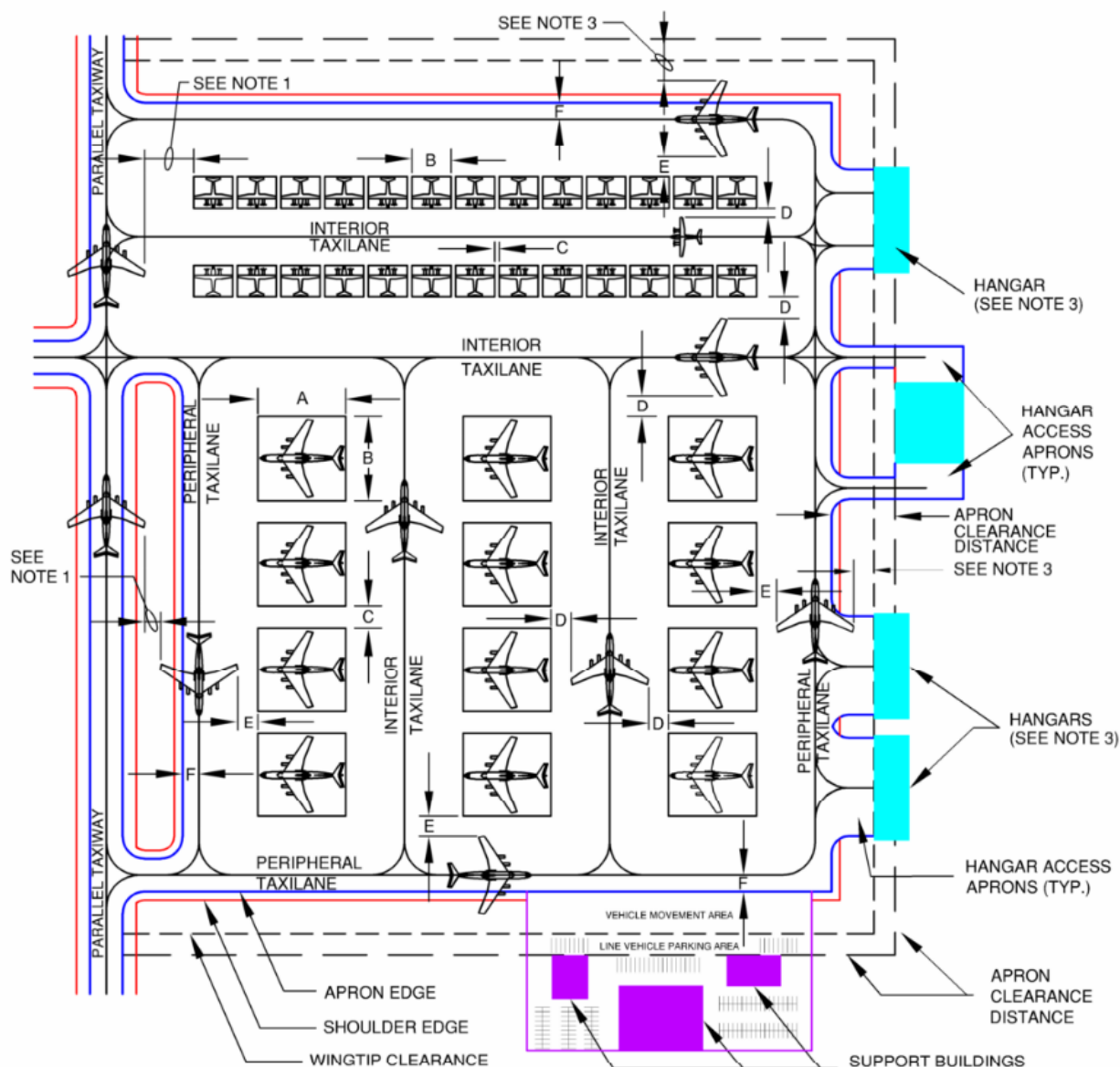
Figure 11320-1 Basic Aircraft Parking Apron
