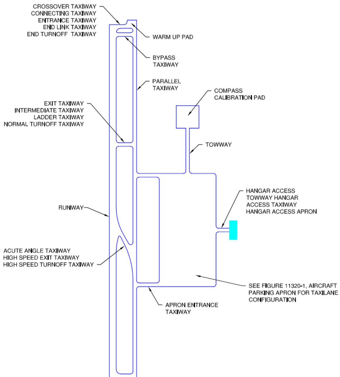
Figure 11210-1 Basic Airfield Layout
