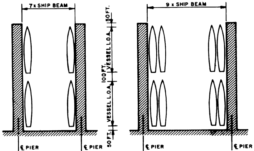
TWO-ABREAST BERTHING
