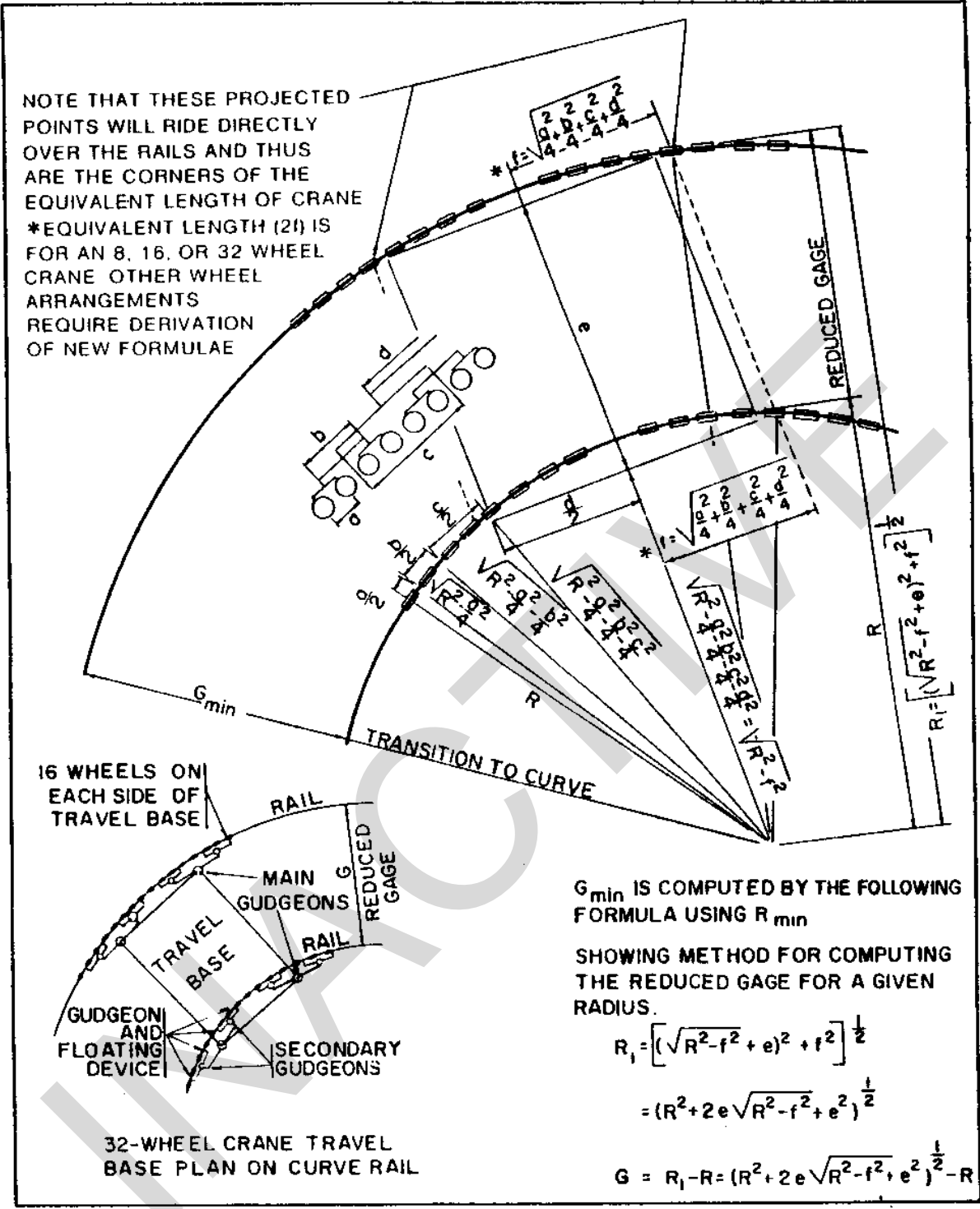
Figure 4 Gage Reduction Diagram (32-Wheel Crane)
