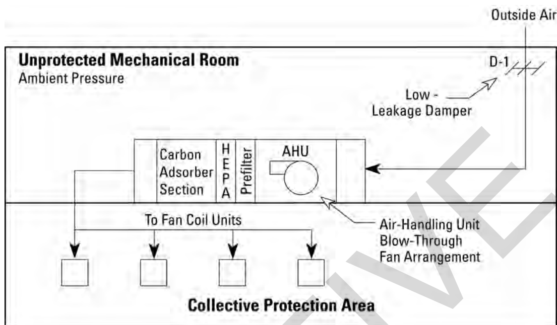
Figure 3-10. Medium Level of Protection – Fan Coil System
