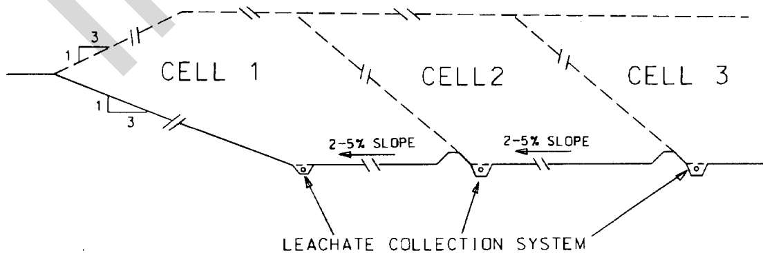
Figure 3-2. Typical Trench Bottom Separated by Berms.
