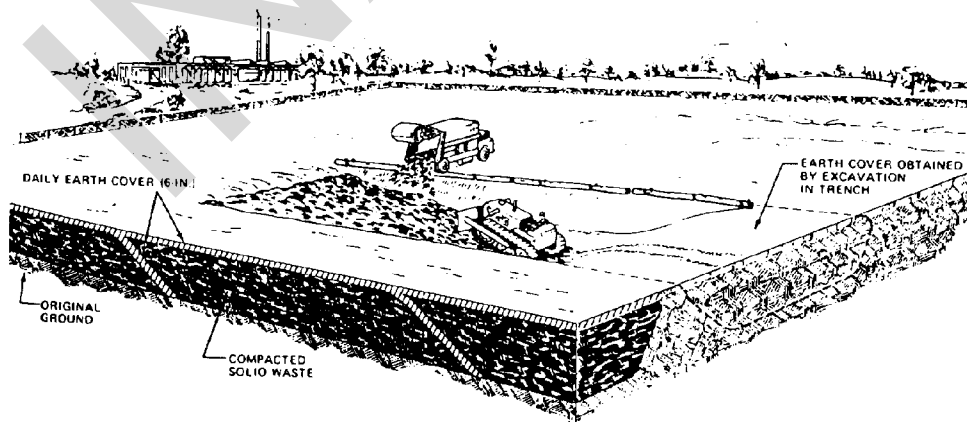
Figure 2-1. Typical Trench Landfill Operation.
