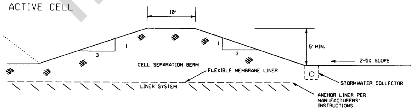
Figure 3-4. Typical Berm Detail.
