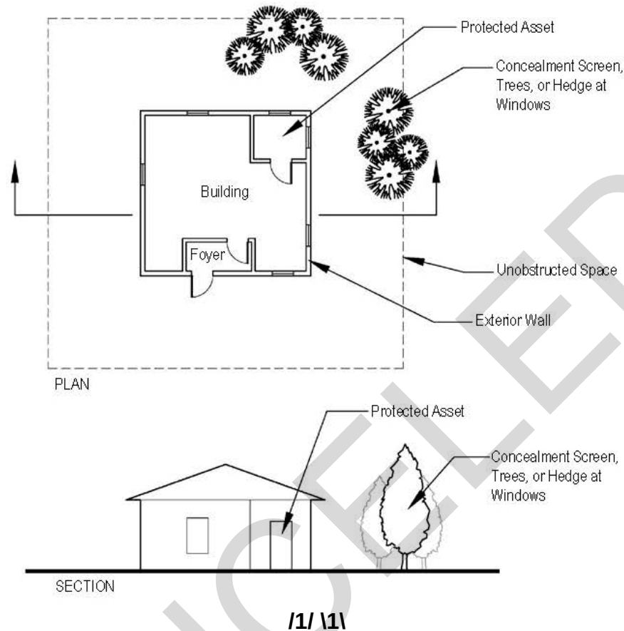
Figure 4-1. Trees and the Unobstructed Space
