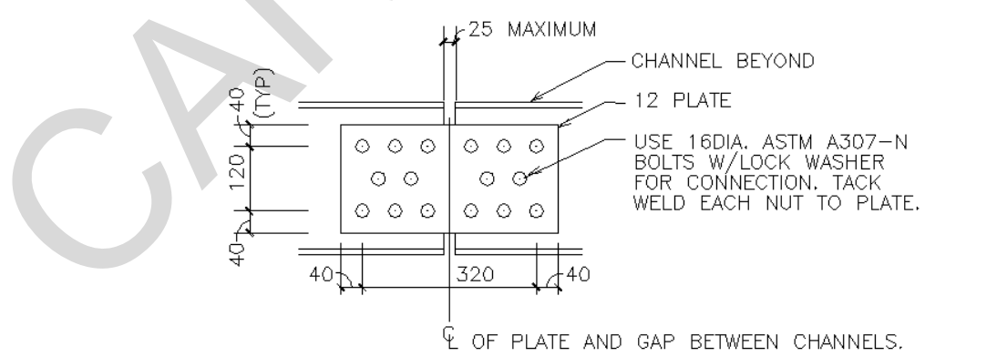
2 CHANNEL SPLICE DETAIL
