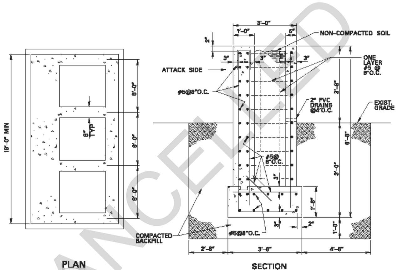
Figure 6-17 Reinforced Concrete Planter
