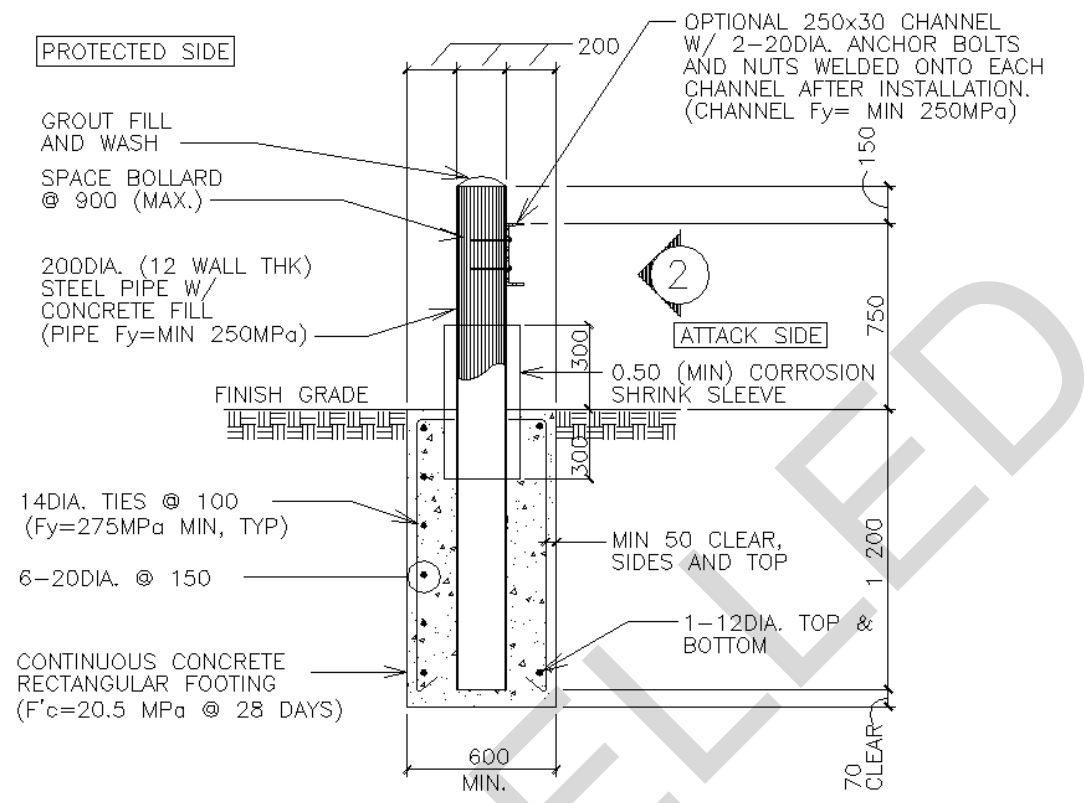
1 BOLLARD SECTION SCALE = 1:20
