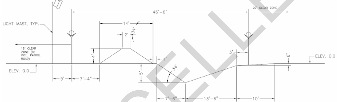
Figure 6-19 Anti-Vehicular Ditch Profile with Maximum Incline Slope Not Requiring Stabilization
