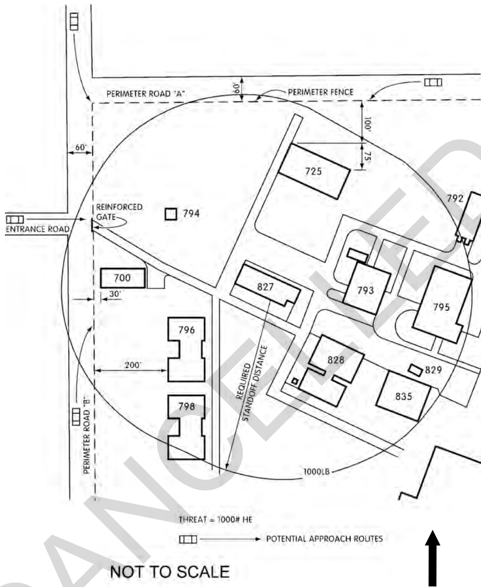
Figure 4-1 Example Site Layout
