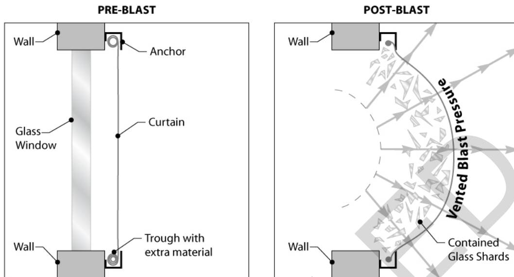
FIGURE 6-5. BLAST CURTAINS
