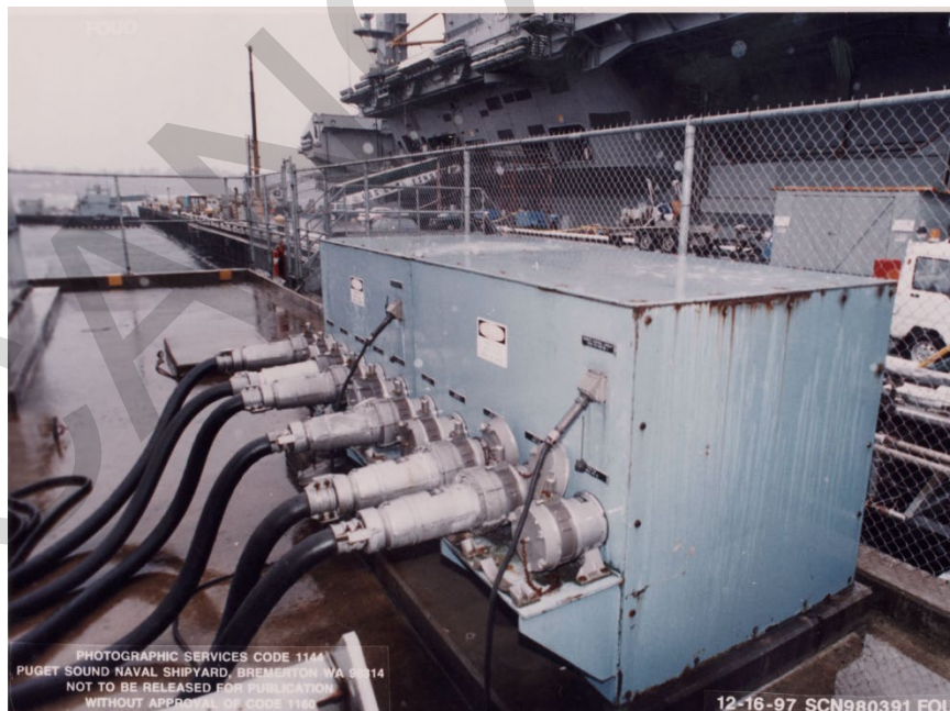
Figure 12-8. 4.16 kV Pier Electrical Outlet Assembly and Outlets – Existing Installations
