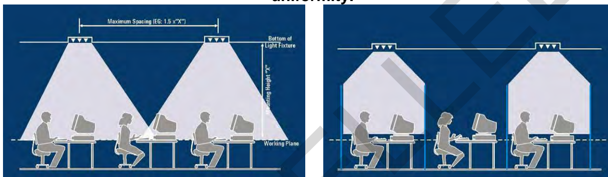
Figure 3-6. A change in furniture configuration affects the task plane illuminance uniformity. 9
