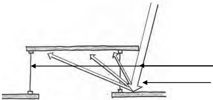
Figure 4-4. Diagrams of Toplighting Strategies.
