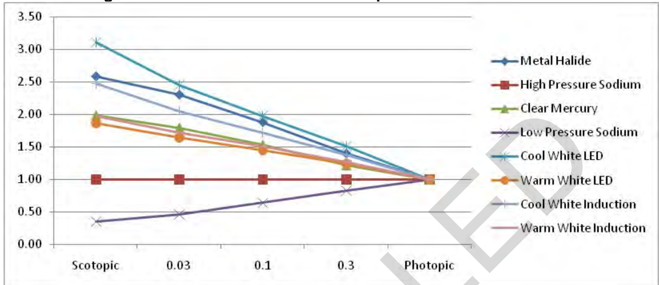
Figure 2-7. Lumen Effectiveness Multipliers vs. Luminance 4
