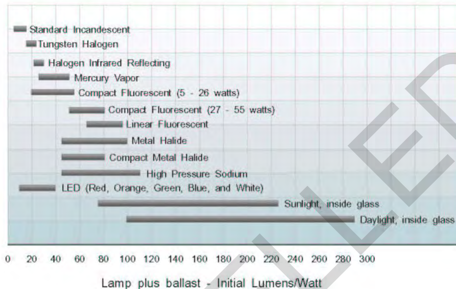
Figure 5-7. Efficacy Comparison of Light Sources for General Lighting.
