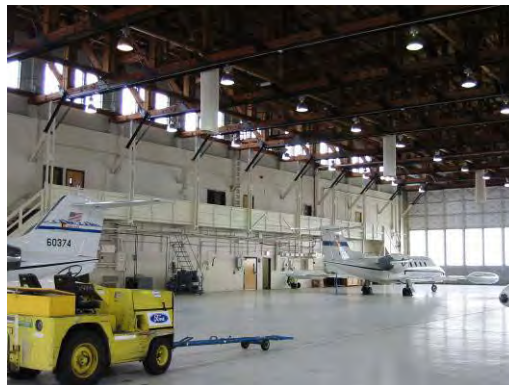
Figure 4-6. Example of Clerestory Application.
