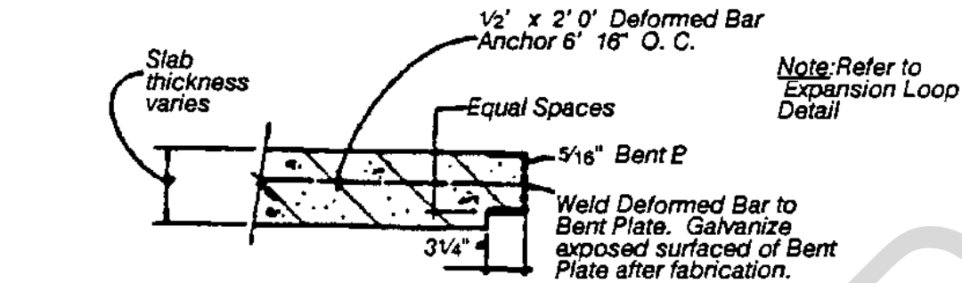
COVER SLAB EDGE REINFORCEMENT AT INTERSECTION
