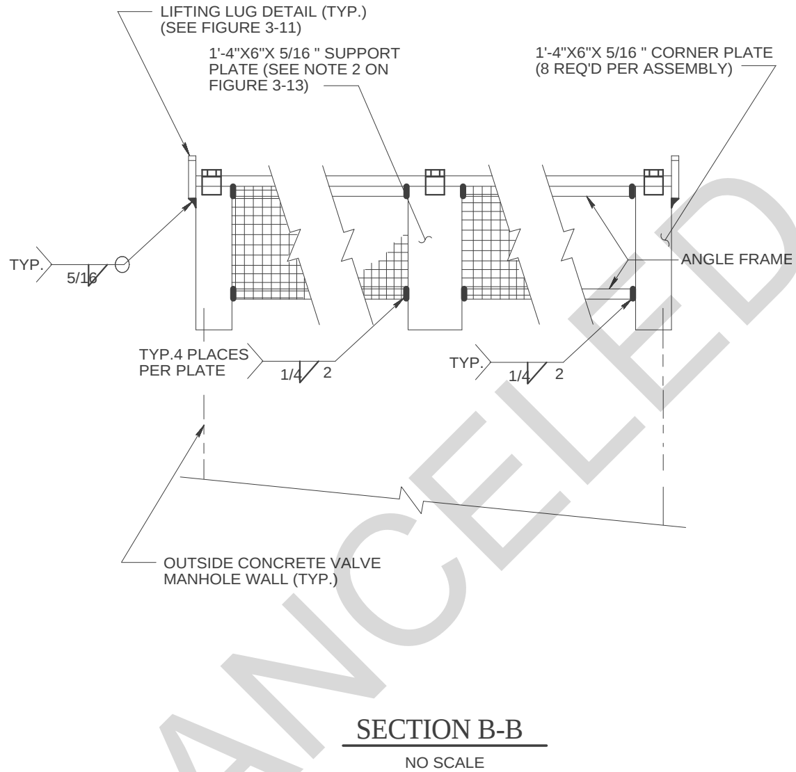
Figure 3-8. Section B-B of Raised Cover Plate.
