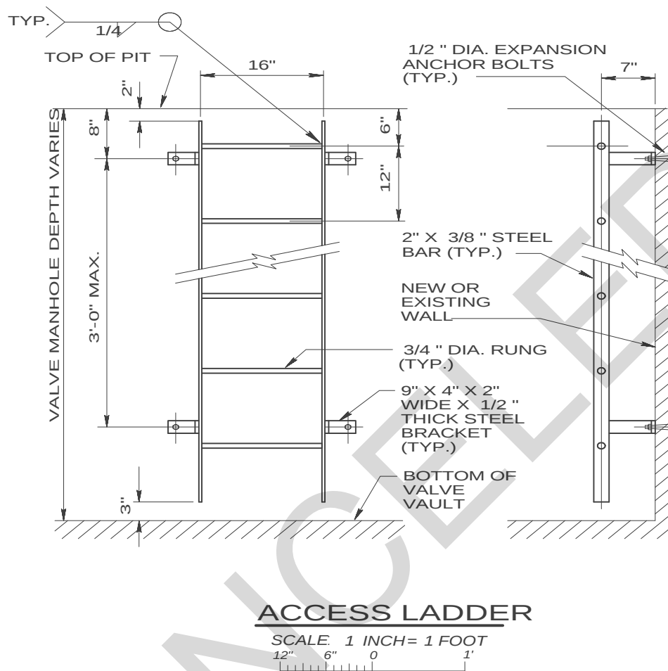
Figure 3-2. Access Ladder Detail.
