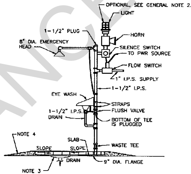
EMERGENCY SHOWER & EYE WASH (ES/EWS) DETAIL N.T.S.
