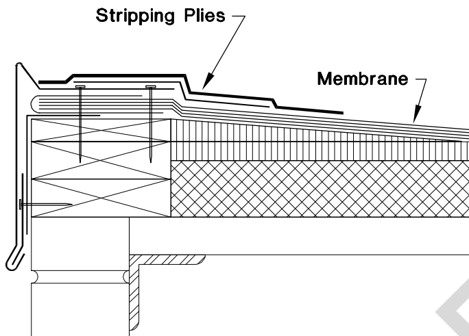
Figure 12-7a. Metal Gravel Stop/Fascia Embedded Between Membrane Plies and Stripping Plies.
