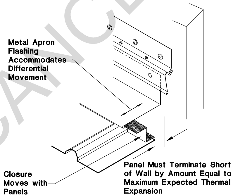
Figure 9-8. Headwall Transition
