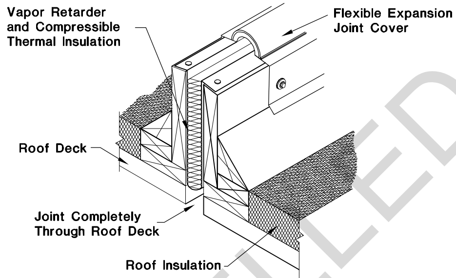
Figure 4-1. Raised Curb Expansion Joint
