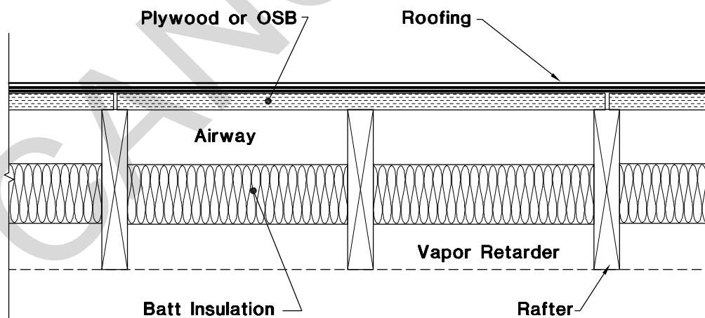
Figure 2-15. Under Deck Insulation
