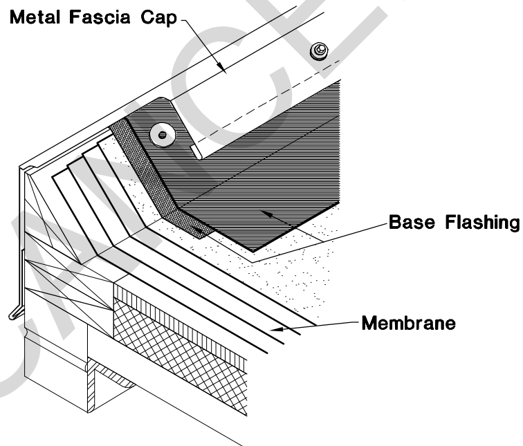
Figure 12-7b. Metal Fascia Cap Placed Over Completed Membrane and Base Flashing.
