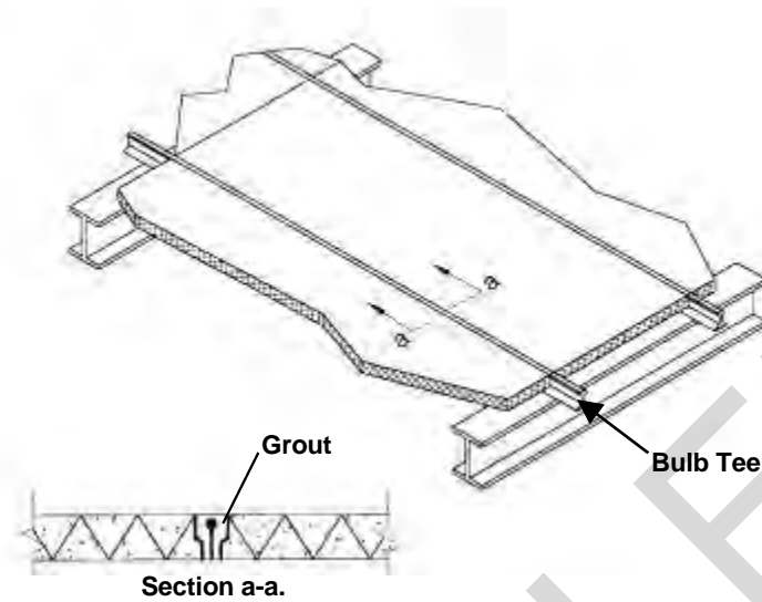
Figure 2-16. Self-Insulating Roof Deck
