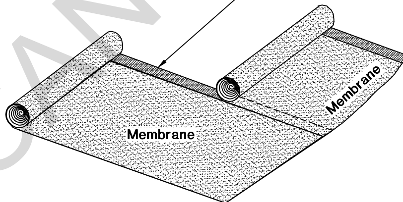
Figure 2-3. Low-Slope (Hydrostatic)
