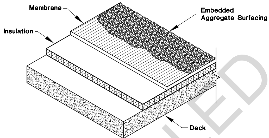
a) Conventional roofing system
