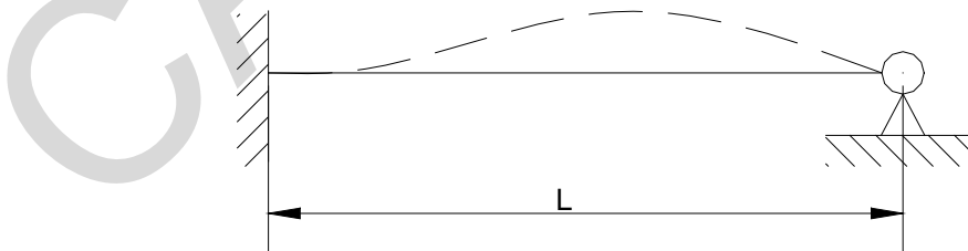
Figure B-7. Fixed-pinned Support Condition for Table B-2
