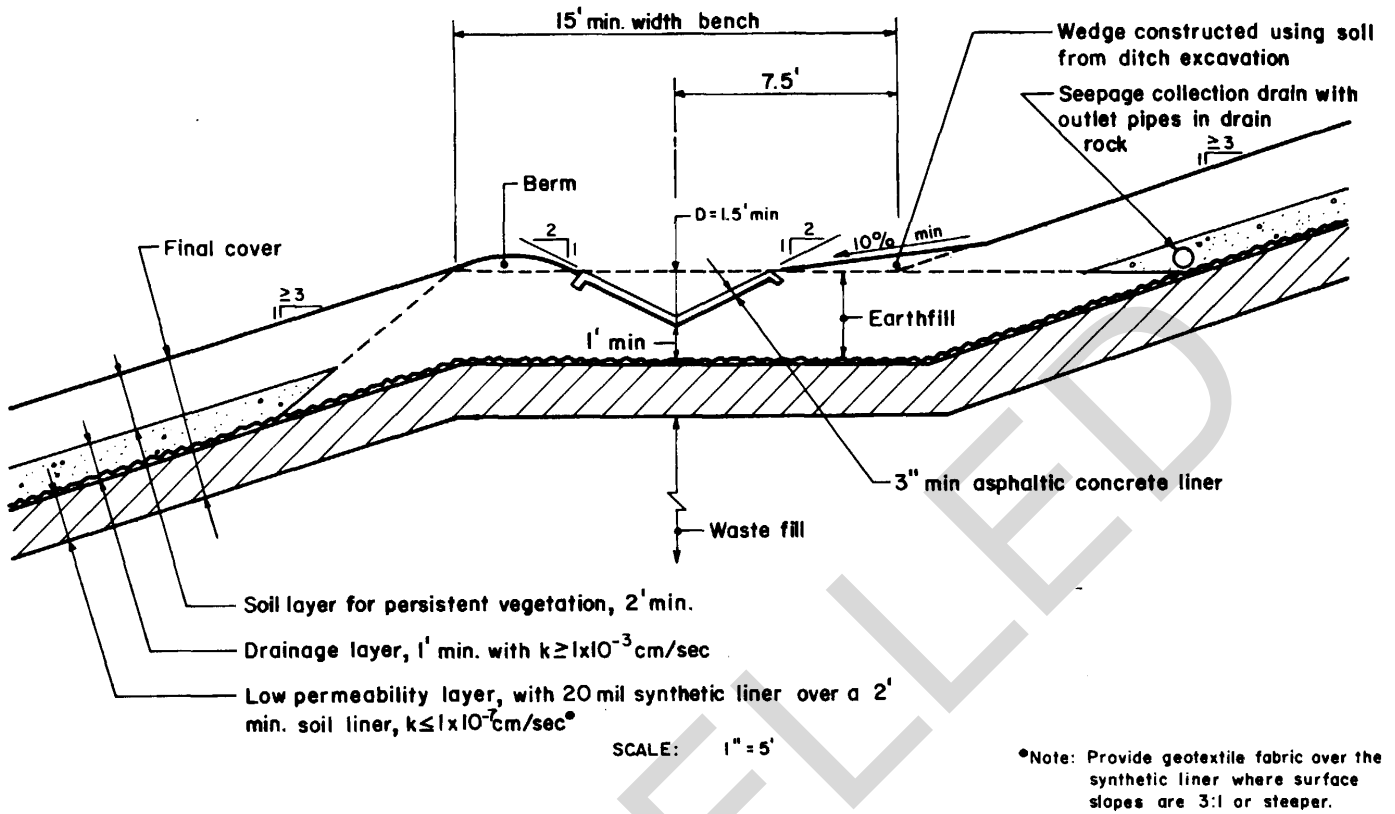
Figure 6-7. Typical run-on control ditch for waste units. 6-17
