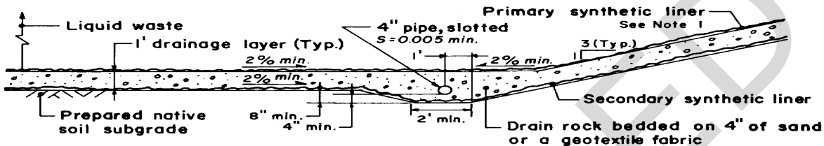
LEAK DETECTION SYSTEM FOR SURFACE IMPOUNDMENT WITH SECONDARY SYNTHETIC LINER
