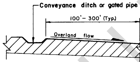
SURFACE IRRIGATION
