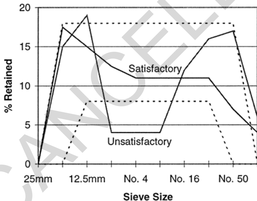
Figure 7-1 Percent Combined Aggregate Retained
