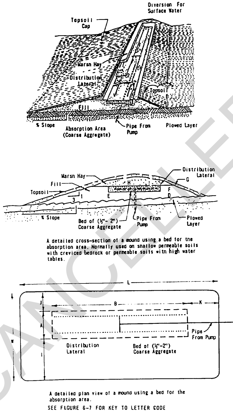
Figure 6-8. Mound system — beds.
