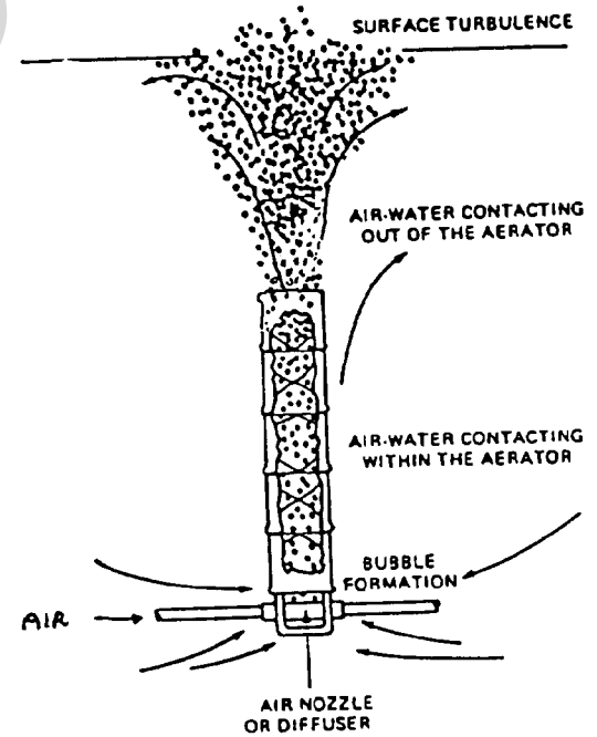
(h) vertical tube diffuser
