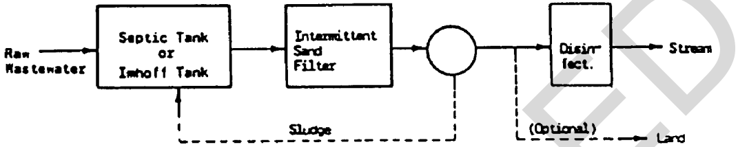
Process Scheme No. 2
