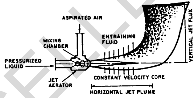
(g) jet aerator
