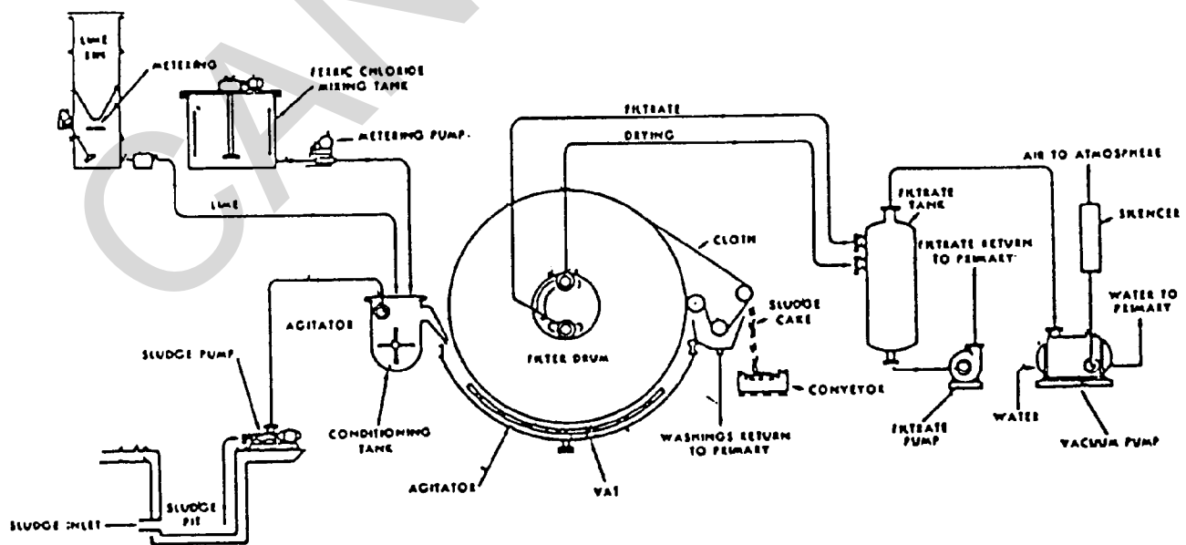
Figure 16-3. Rotary vacuum filter system.
