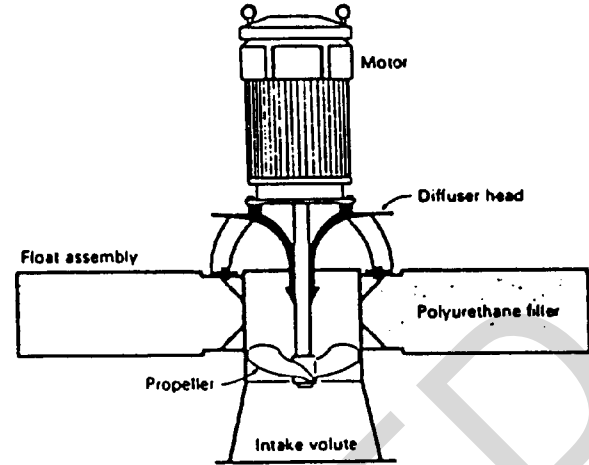
(f) floating mechanical surface aerator
