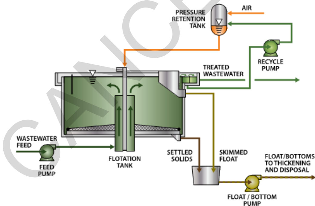
Figure 10-3 Process Schematic of Dissolved Air Flotation
