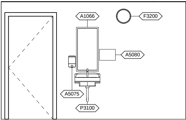
XDM01 - SOUTH ELEVATION
