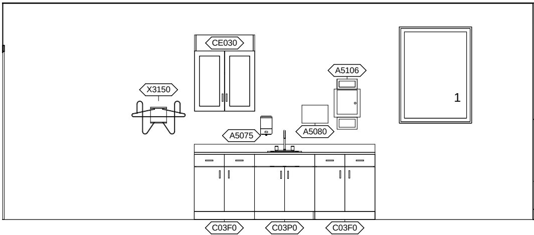
XDCY1 - EAST ELEVATION
