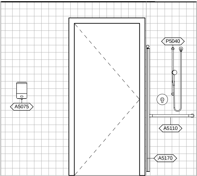
TLTS1 - WEST ELEVATION
