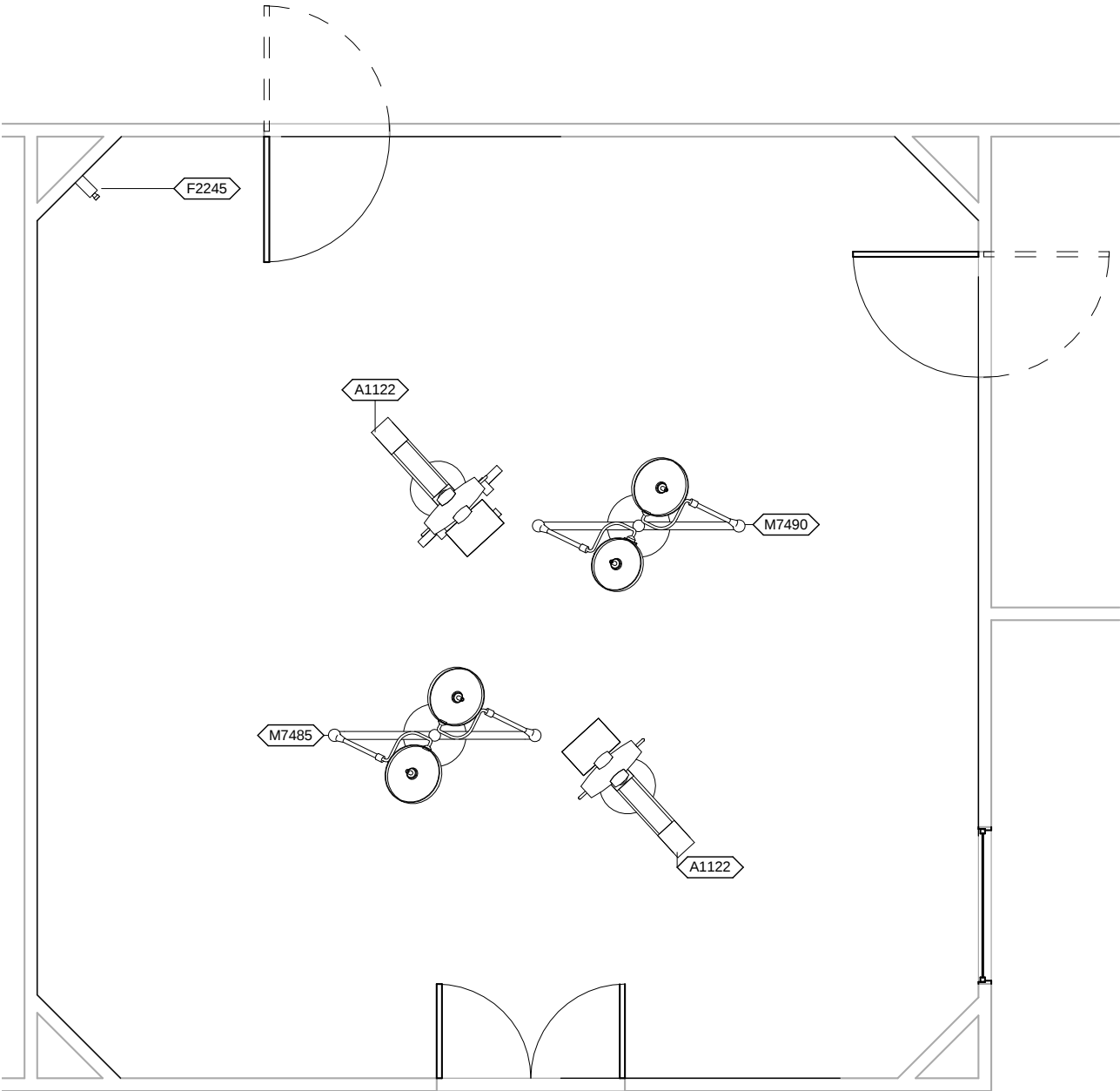
ORNS1 - CEILING MOUNTED EQUIPMENT PLAN
