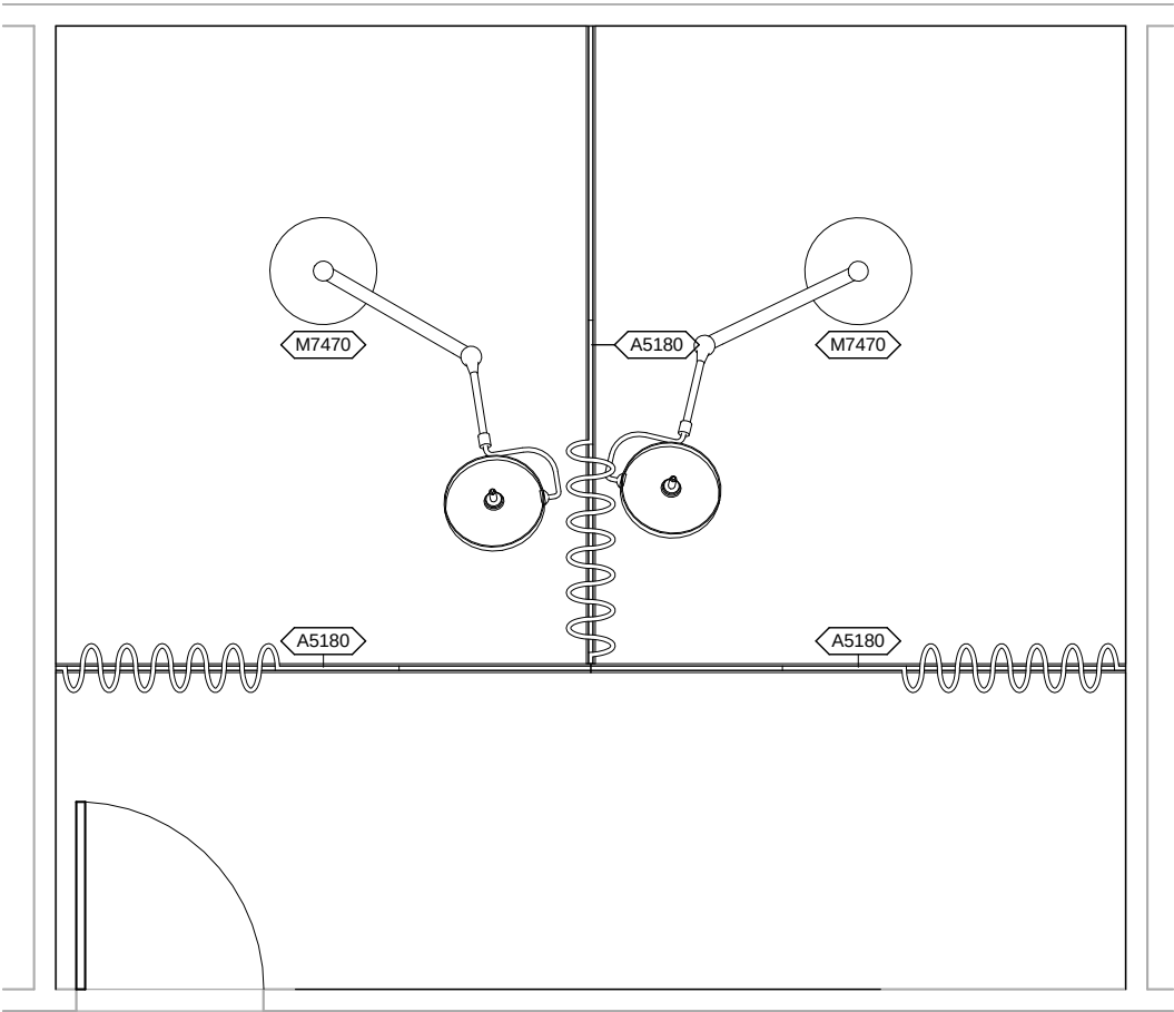
OPCR2 - CEILING MOUNTED EQUIPMENT PLAN
