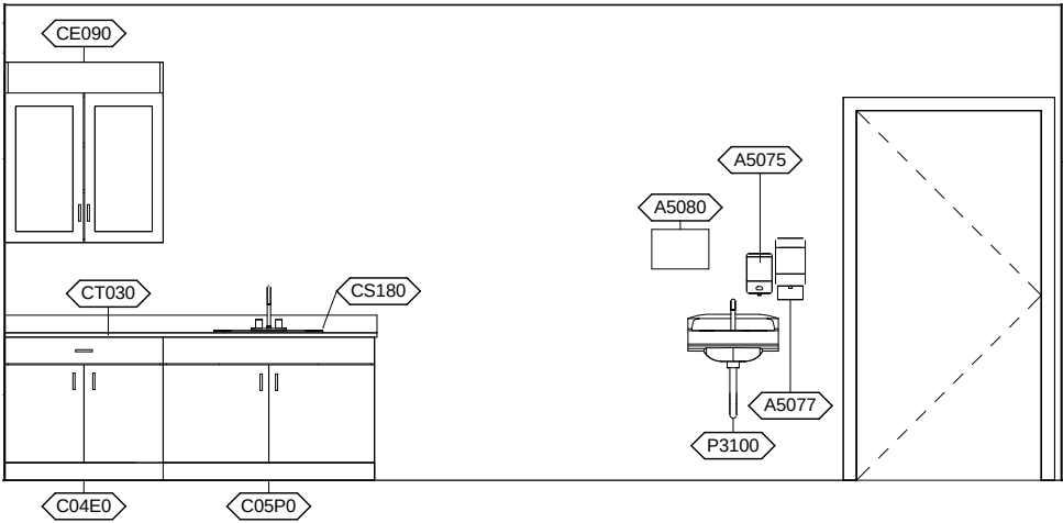
OPCR2 - SOUTH ELEVATION
