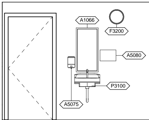
EYVS1 - SOUTH ELEVATION
