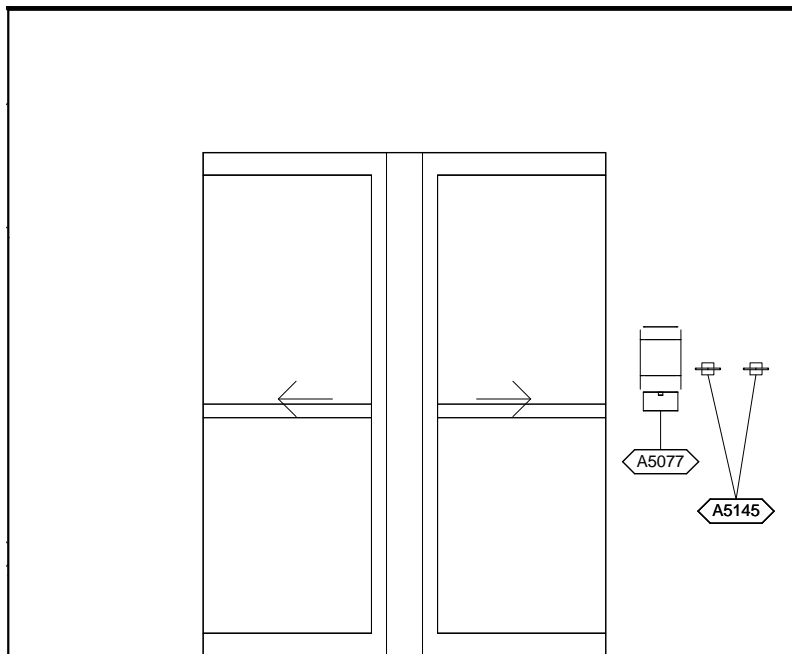
EXER1 - SOUTH ELEVATION
