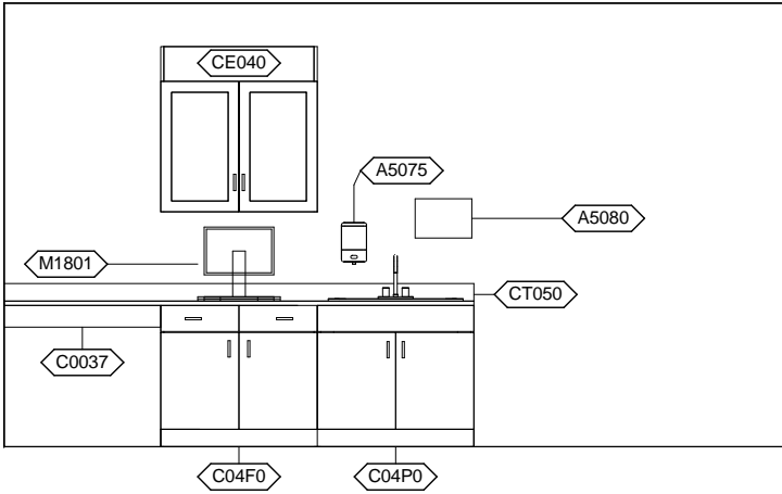
DNSC4 - NORTH ELEVATION
