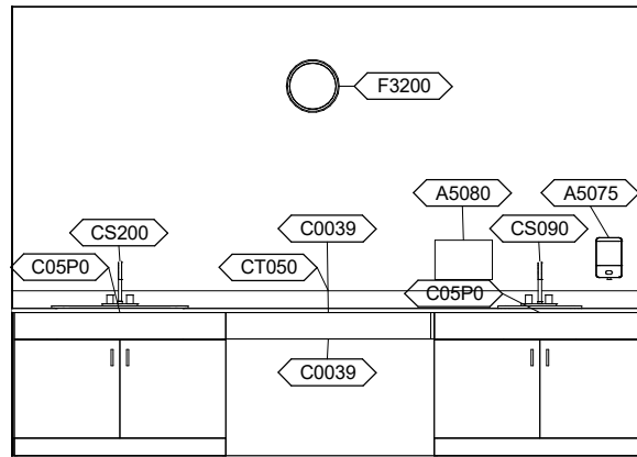
DNPL1 - EAST ELEVATION
