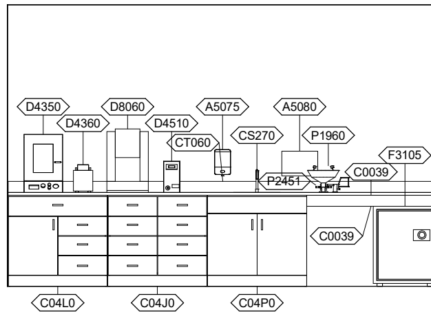
DNPC1 - WEST ELEVATION
