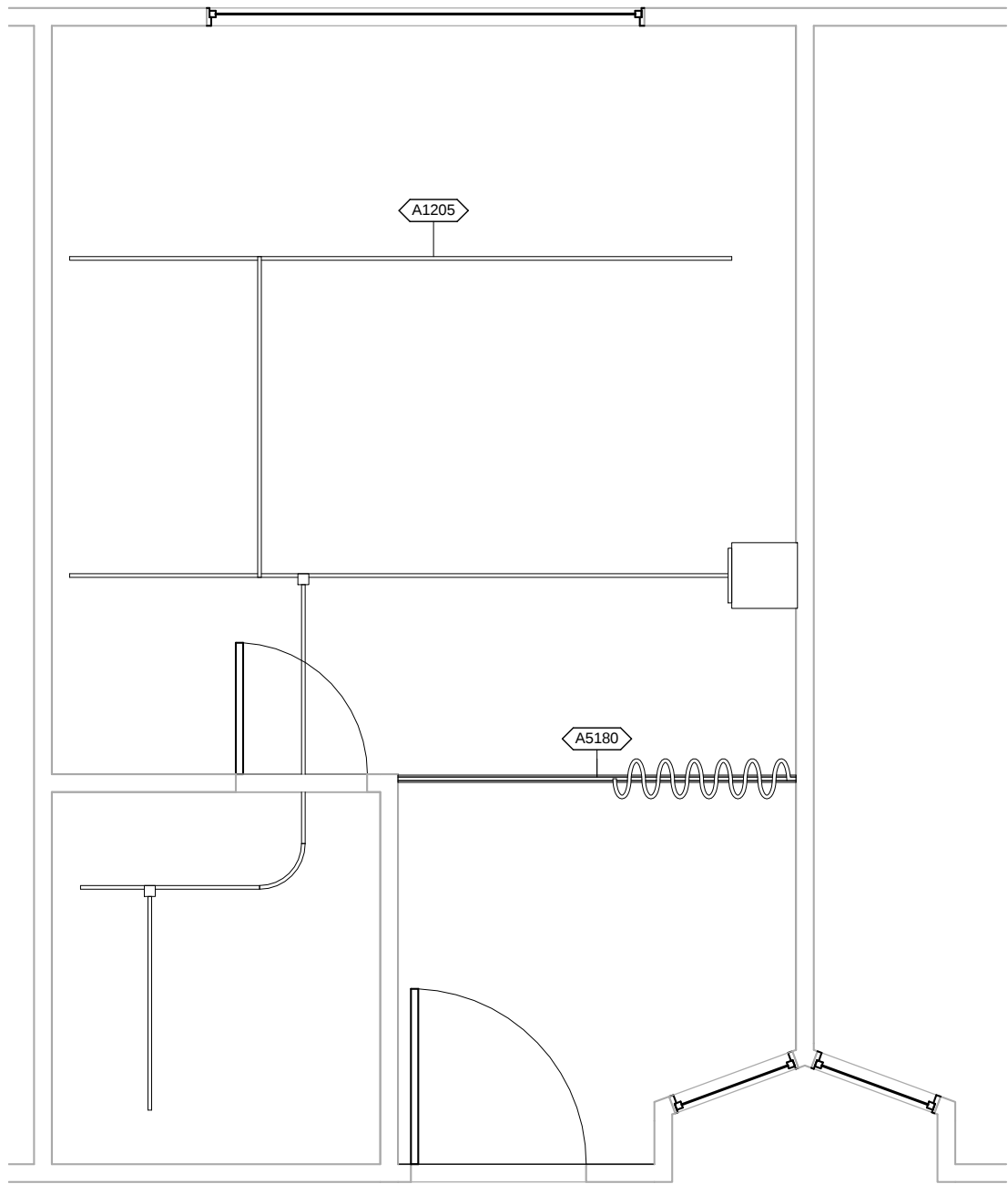
BRMS1 - CEILING MOUNTED EQUIPMENT PLAN
