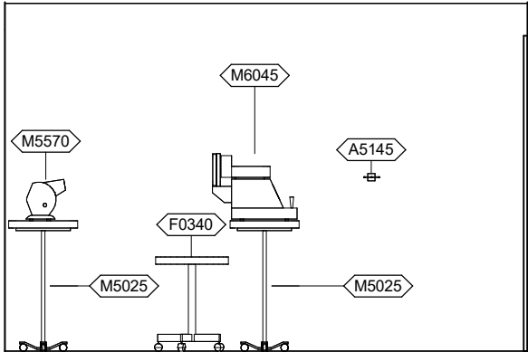
EYVS1 - EAST ELEVATION
