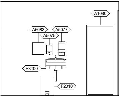
EXRG1 - EAST ELEVATION
