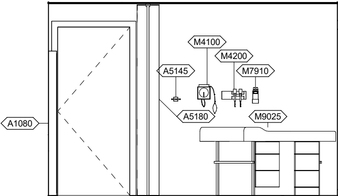
EXRG1 - SOUTH ELEVATION
