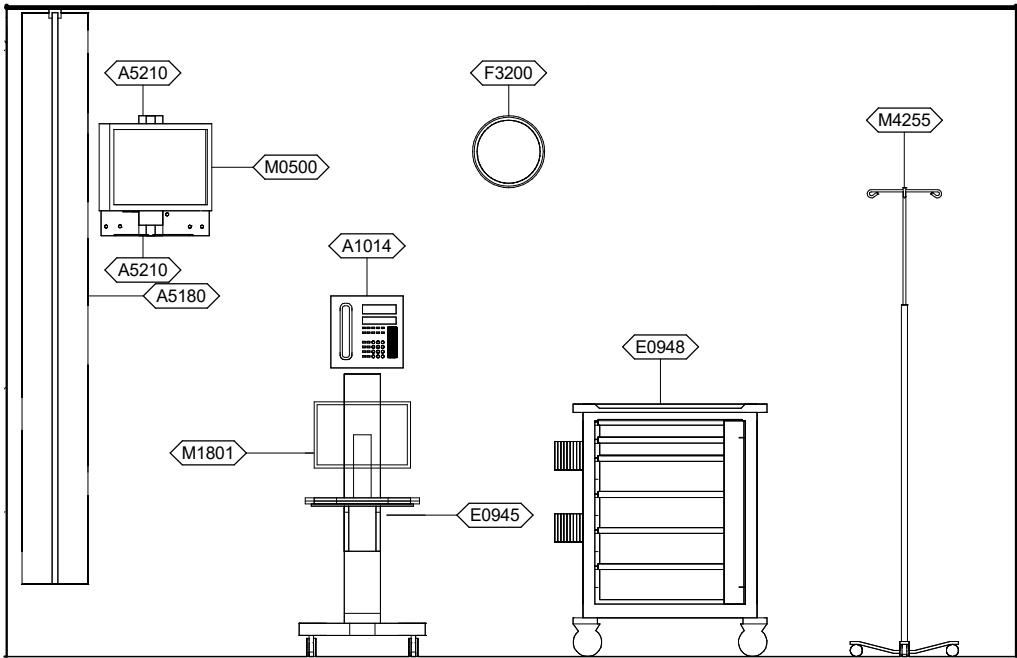
EXER1 - WEST ELEVATION
