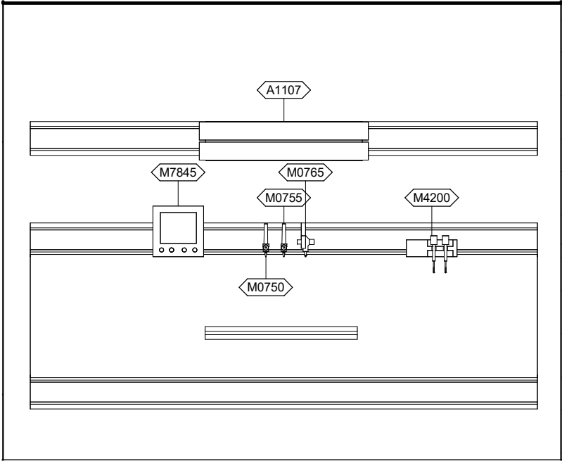
EXER1 - NORTH ELEVATION
