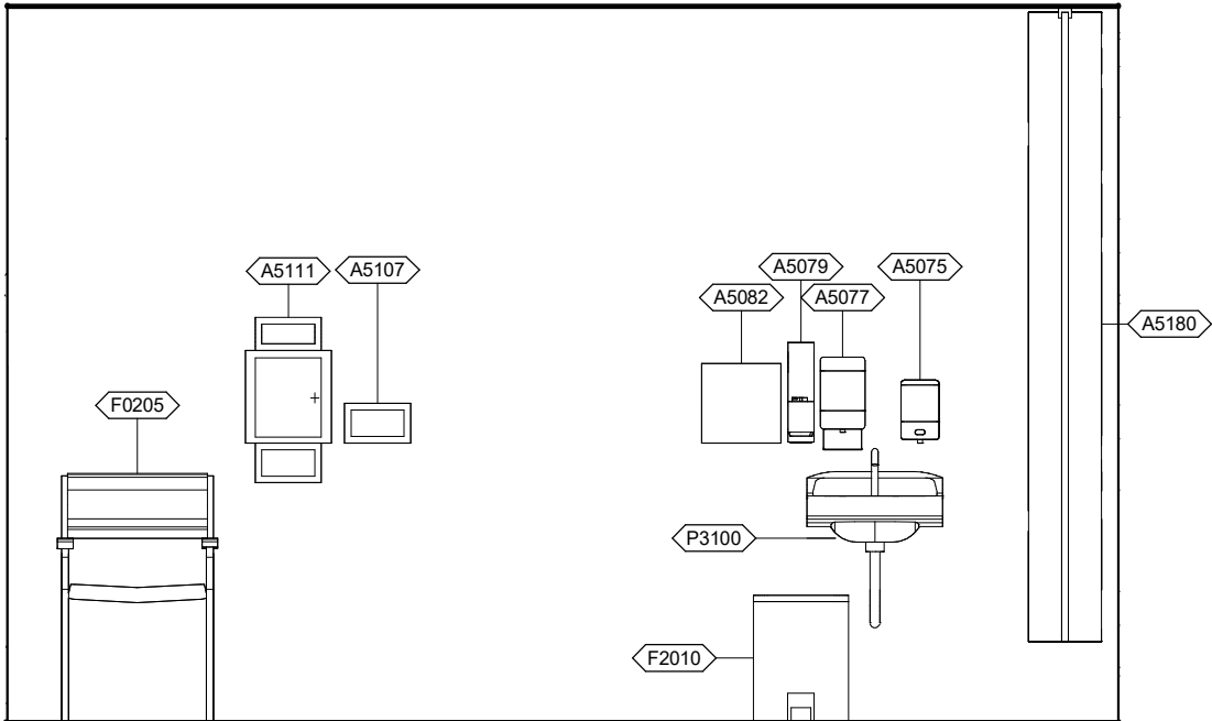
EXER1 - EAST ELEVATION
