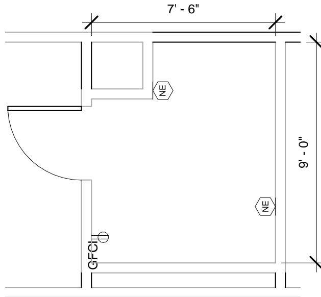
TLTS1 - FLOOR PLAN
