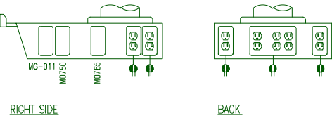
A1120_PREFAB SURGICAL SERVICE COLUMN.
