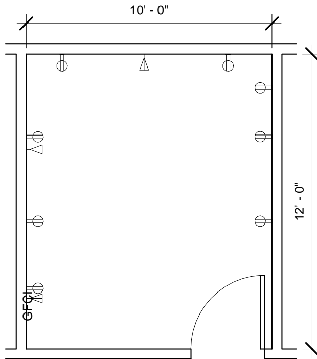
OFD02 - FLOOR PLAN
