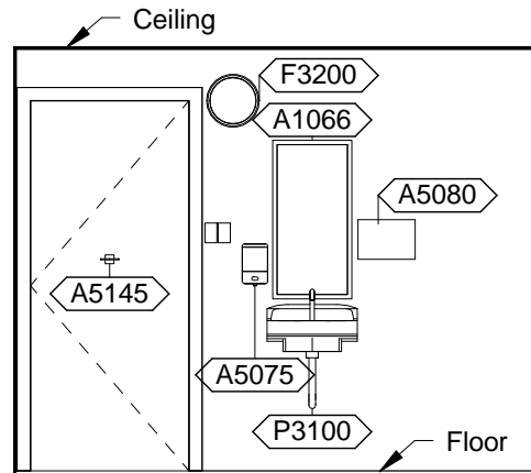
OFD01 - PLAN SOUTH
