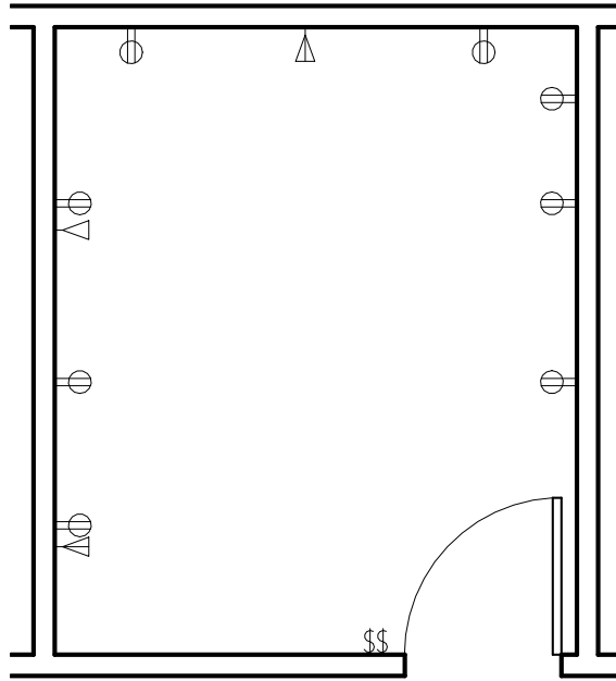
OFD01 - FLOOR PLAN
