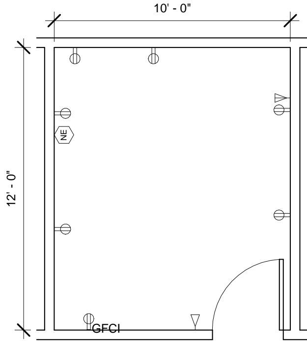
NMUR1 - FLOOR PLAN
