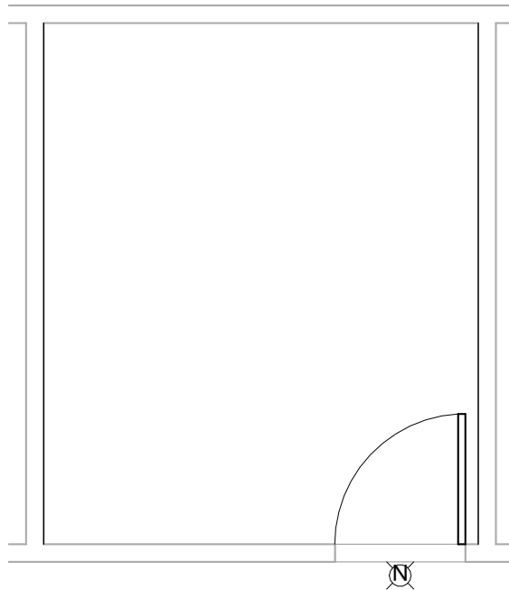
NMUR1 - CEILING MOUNTED EQUIPMENT PLAN
