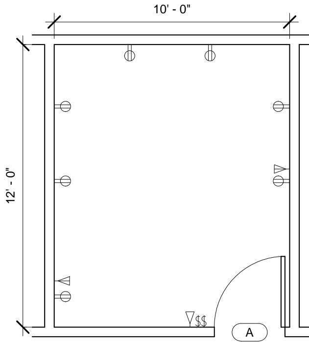
EXEN1 - FLOOR PLAN
