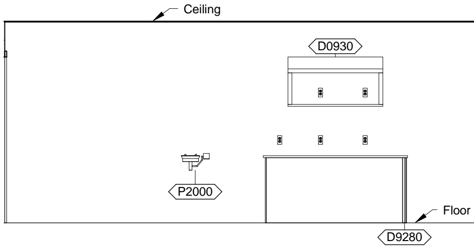
DNPL2 - PLAN NORTH
