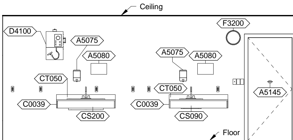
DNPL2 - PLAN SOUTH
