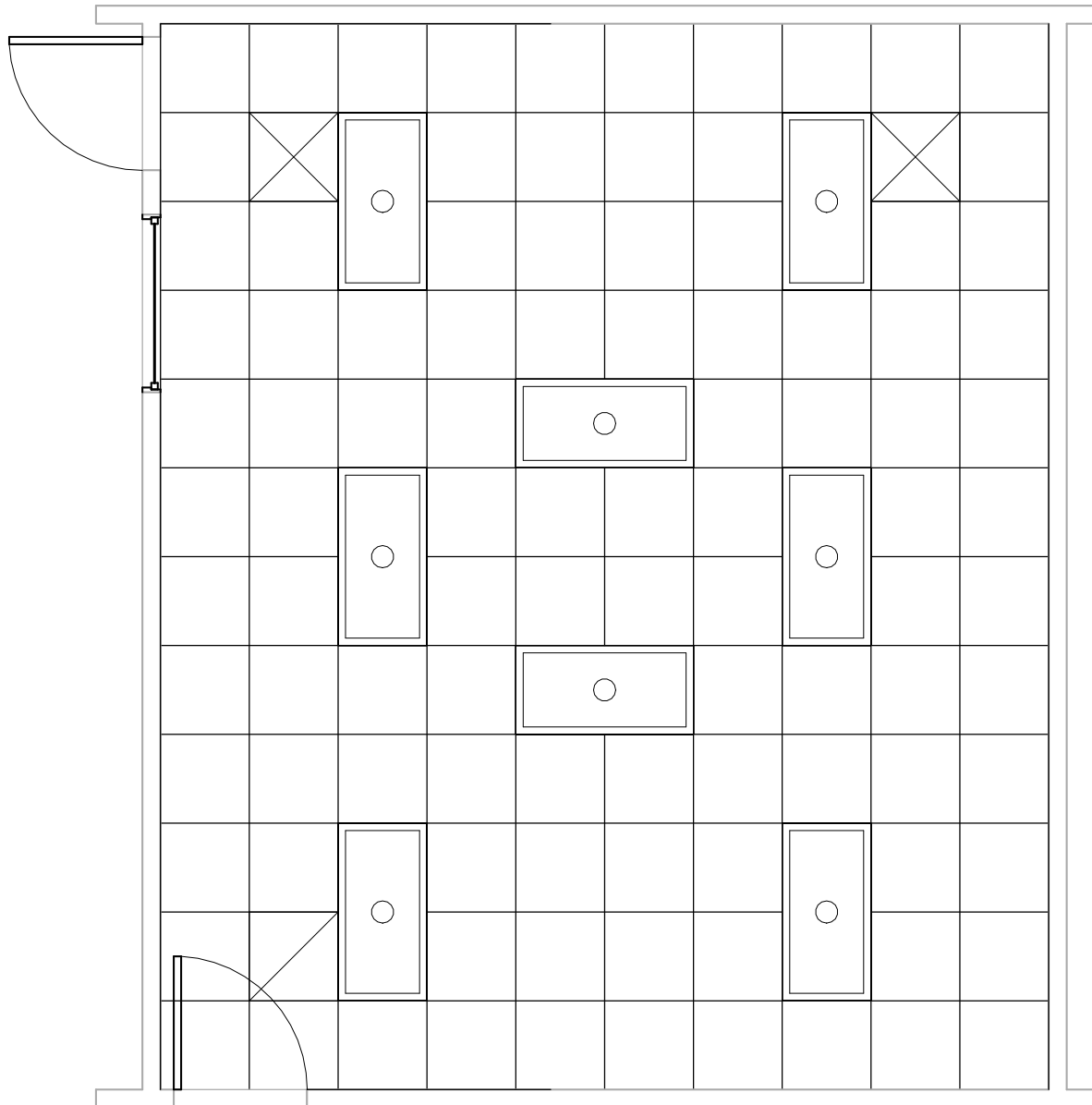
DNPL2 - CEILING PLAN
