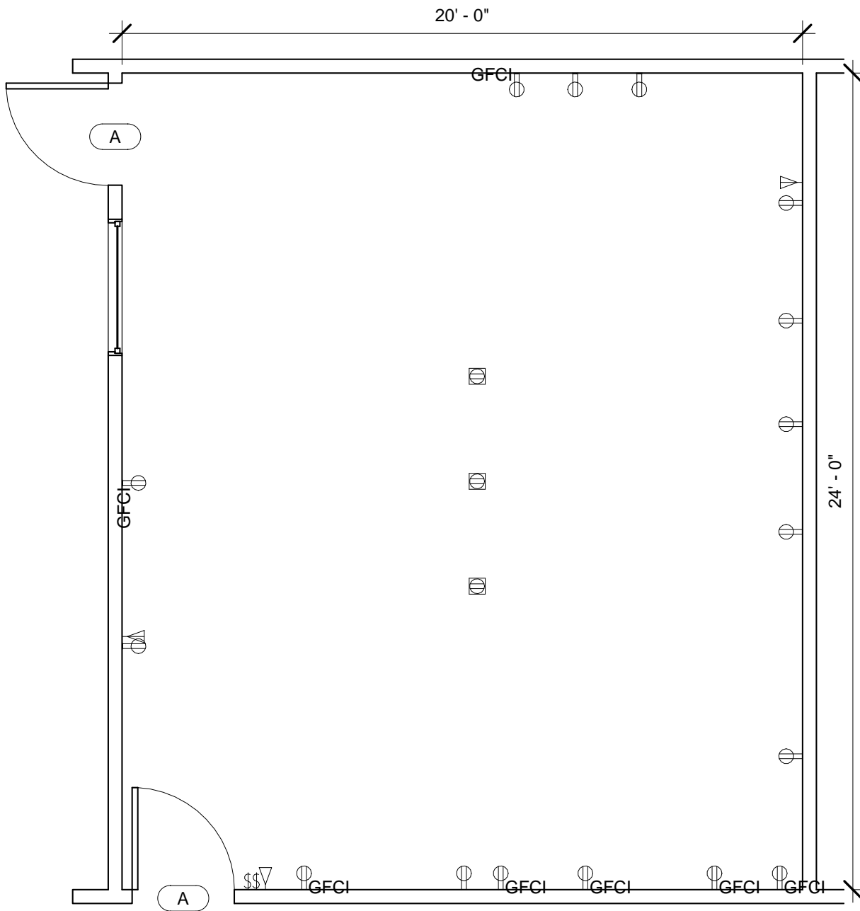
DNPL2 - FLOOR PLAN
