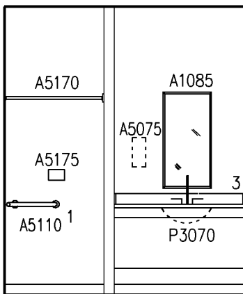
SOUTH (BATHROOM)
